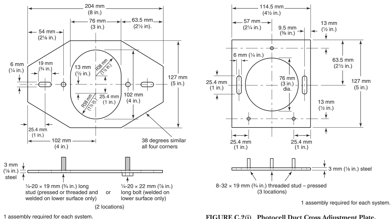
FIGURE C.2(i) Photocell Duct Inline Adjustment Plate.
