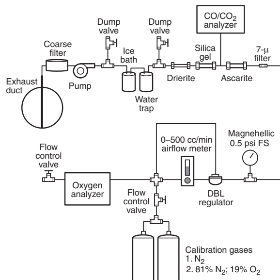
FIGURE B.4.1.2 Schematic of Gas Sampling System.
