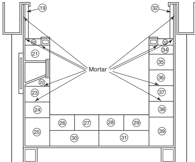
FIGURE C.1(c) Cross-Section of the Fire Test Chamber.
