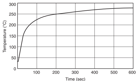
FIGURE 6.6.5.1 Representative Test Flame Temperature History Curve.
