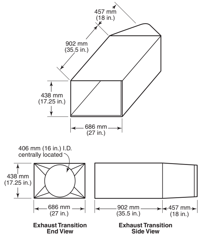
FIGURE 4.2.6.1.1 Exhaust Transition. Tolerances are contained in applicable paragraphs. Otherwise, dimensions are nominal.
