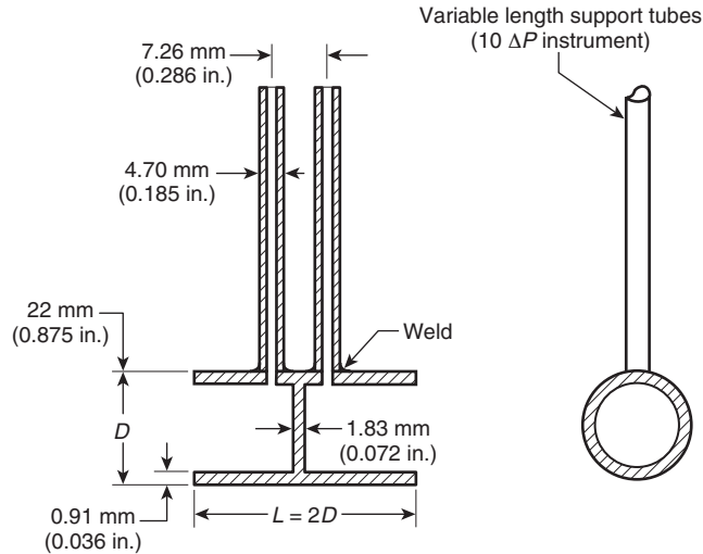
FIGURE 4.2.8.1.1 Bidirectional Probe.
