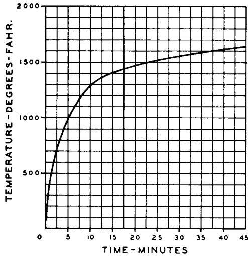
Figure 2-1.1 Time-Temperature Curve
