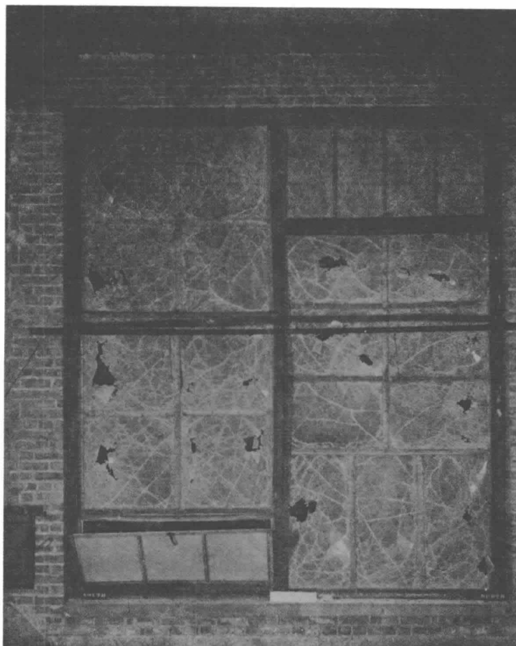
Figure 6-1 Unexposed Side of Window Assembly after Fire Exposure and Hose Stream Application.
