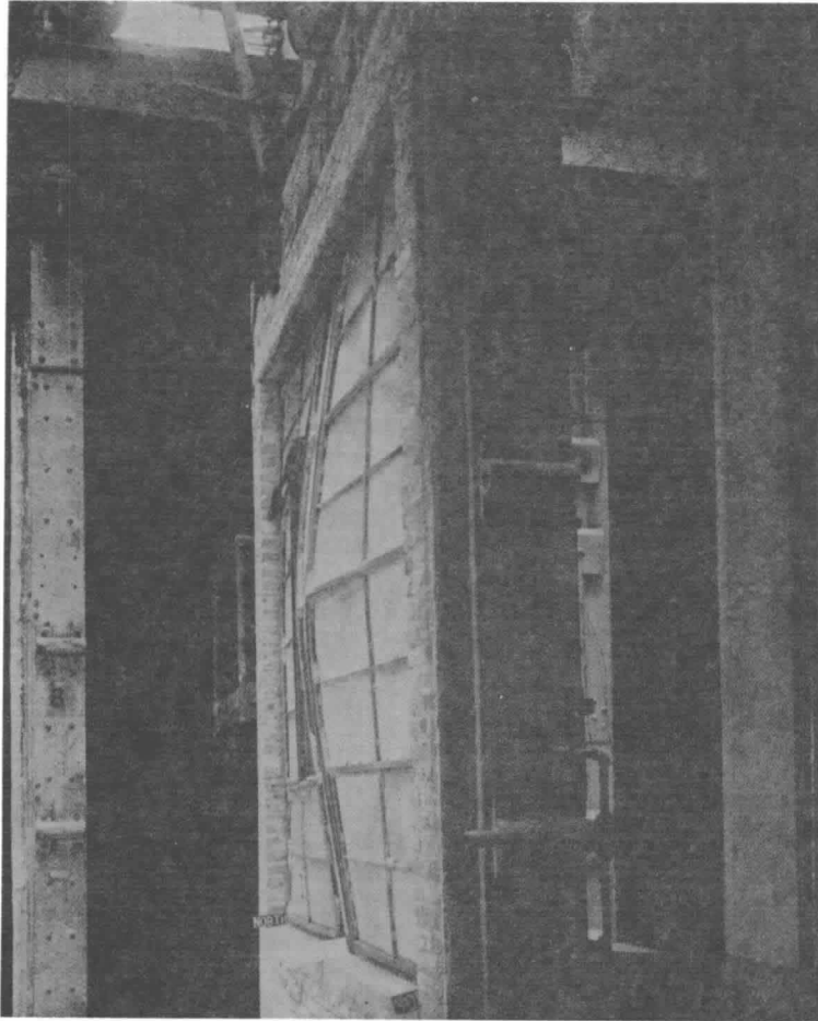
Figure 6-2 Exposed Side of Window Assembly after Fire Exposure and Hose Stream Application.
