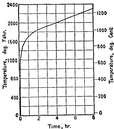
Fig. 1. Time Temperature Curve.
