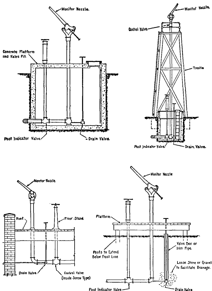
Fig. 71. Standard Monitor Nozzles.
