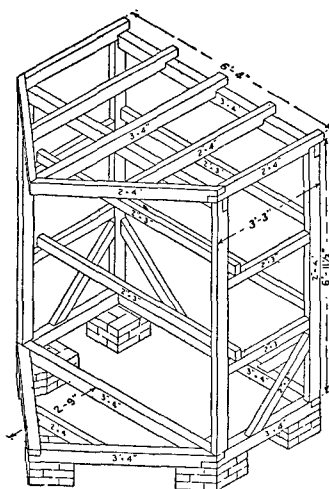
Fig. 53-2. Typical Hose House Framing Plan
