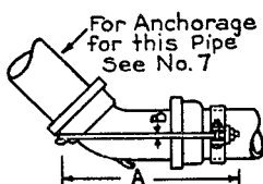
No. 4 1/8 BEND ANCHOR
