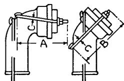
No. 10 PLUG CLAMP BELL END 1/4 & 1/8 BENDS
