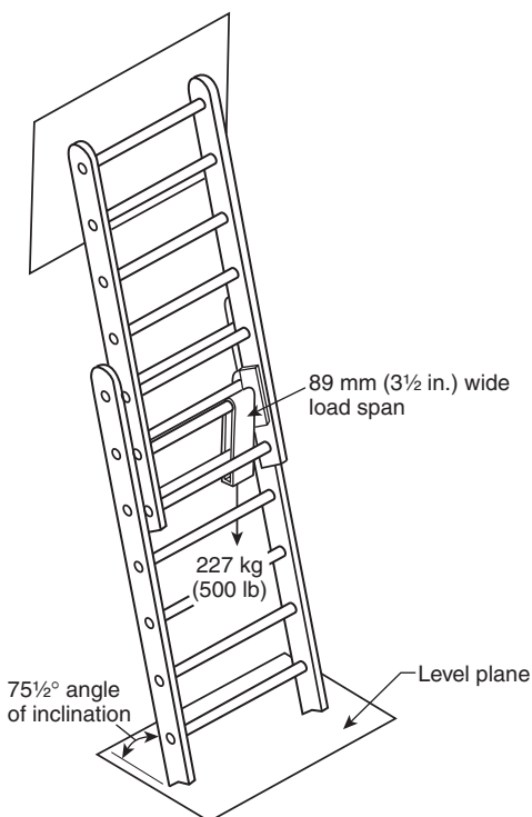
FIGURE 5.2.2.1 Position of Ladder During Design Verification Deflection Test.
