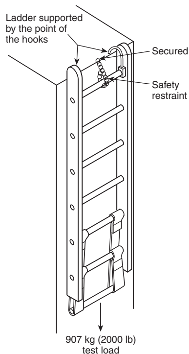
FIGURE 5.3.1 Design Verification Roof Hook Test.
