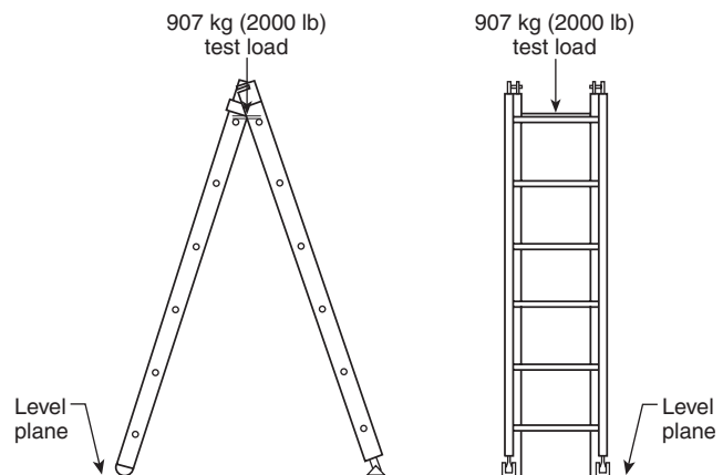
FIGURE 5.6.2.1 Design Verification Combination Ladder Compression Test.
