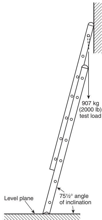
FIGURE 5.4.1.2 Design Verification Beam and Hardware Load Test.
