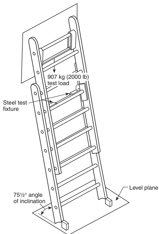
FIGURE 5.4.3.2 Design Verification Pawl Tip Load Test.
