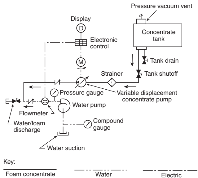
FIGURE A.21.2.6(a) Single-Meter Flow-Sensing Direct Injection Foam Proportioning System.
