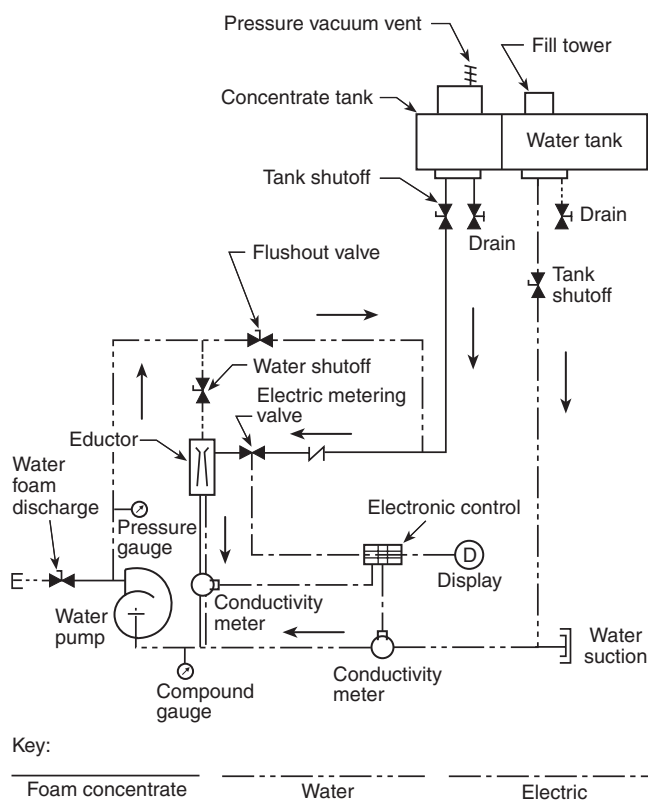
FIGURE A.21.2.4(c) Conductivity-Sensing Automatic Variable Metering Around-the-Pump Proportioning System.
