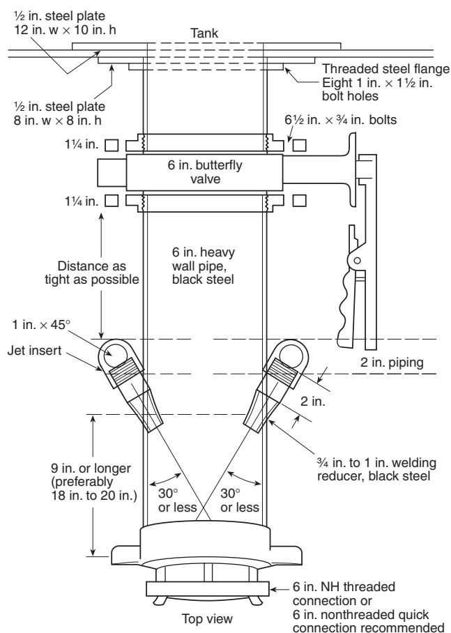
FIGURE A.19.5.2.2(b) Peripheral Jet Assist Arrangement (Top View).
