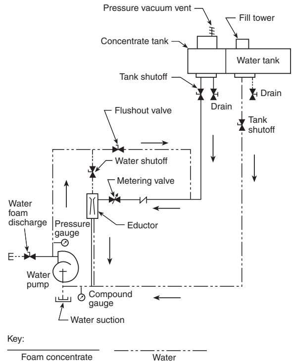
FIGURE A.21.2.4(a) Manual Around-the-Pump Proportioning System.
