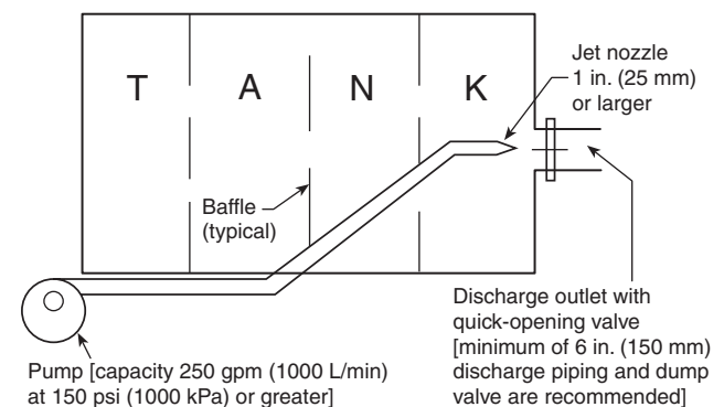
FIGURE A.19.5.2.2(a) Traditional Internal Jet Dump.
