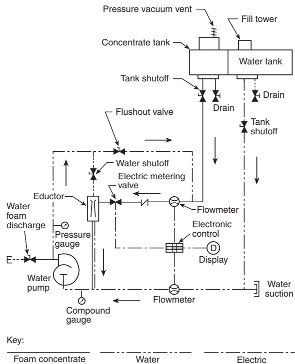
FIGURE A.21.2.4(b) Flowmeter Sensing Around-the-Pump Proportioning System.
