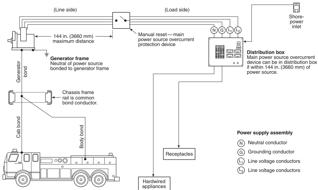
FIGURE A.23.1 Typical Line Voltage Electrical System.
