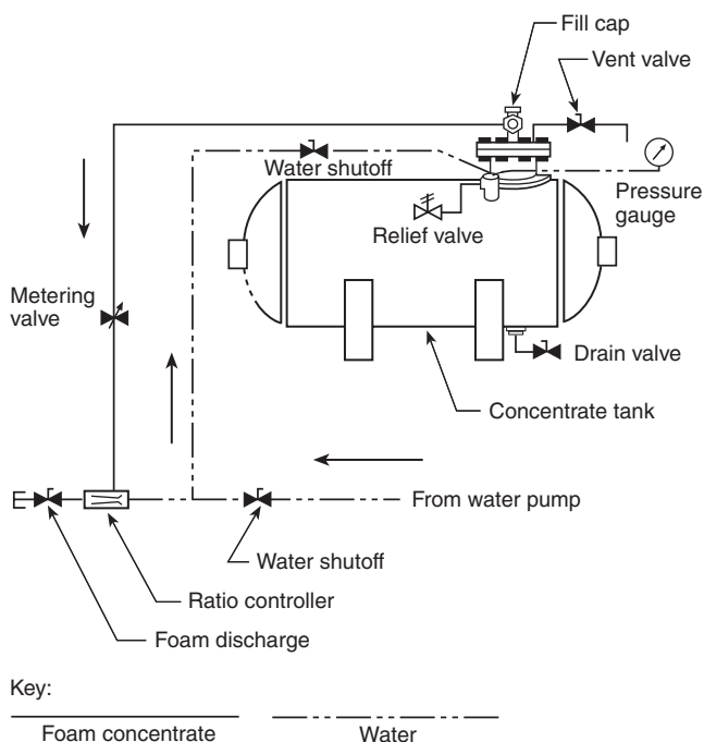
FIGURE A.21.2.5(a) Pressure Proportioning Balanced Pressure Proportioning System.
