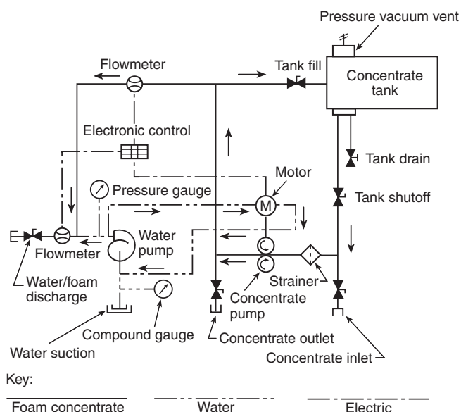
FIGURE A.21.2.7(b) Water Turbine-Driven Flow-Sensing Direct Injection Foam Proportioning System.
