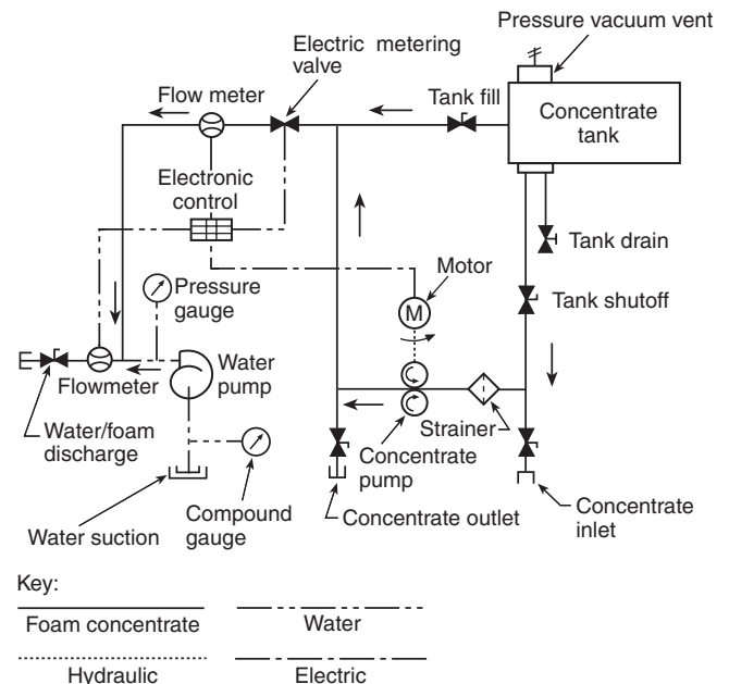
FIGURE A.21.2.6(b) Dual-Meter Flow-Sensing Direct Injection Foam Proportioning System.
