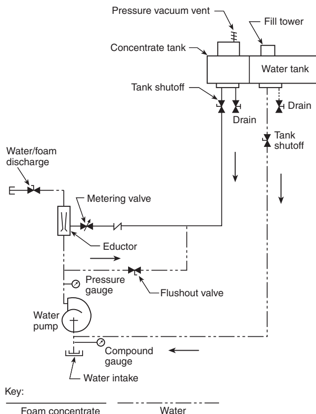
FIGURE A.21.2.1(a) In-Line Eductor Foam Proportioning System.
