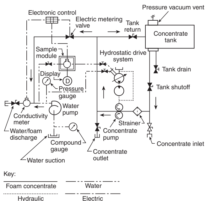
FIGURE A.21.2.6(c) Conductivity-Sensing Direct Injection Foam Proportioning System.
