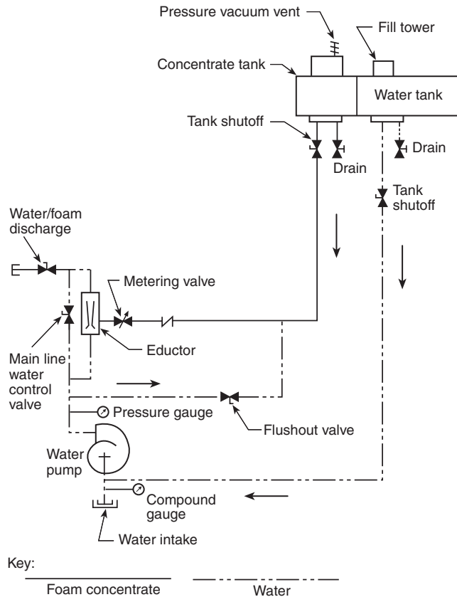
FIGURE A.21.2.1(b) Variable Flow Bypass Eductor System.
