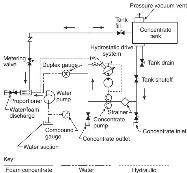
FIGURE A.21.2.5(c) Demand Balanced Pressure Proportioning System.
