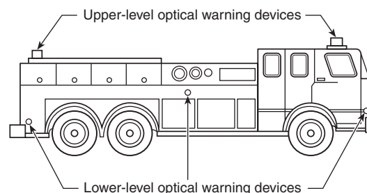
FIGURE A.13.8.1 Upper- and Lower-Level Optical Warning Devices.
