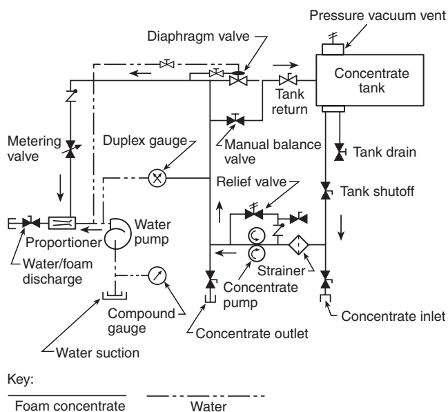
FIGURE A.21.2.5(b) Bypass Balanced Pressure Proportioning System.
