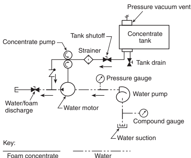
FIGURE A.21.2.7(a) Water Motor Foam Proportioning System.
