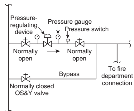
FIGURE A.7.2.2(a) Pressure-Regulating Device Arrangement.
