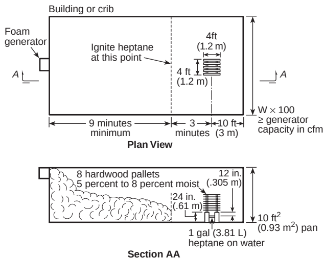
Figure A-1-10.5(a) Fire performance test.
