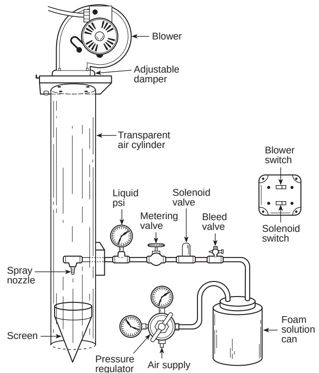
Figure A-1-10.5(b)(1) High-expansion foam quality test generator.
