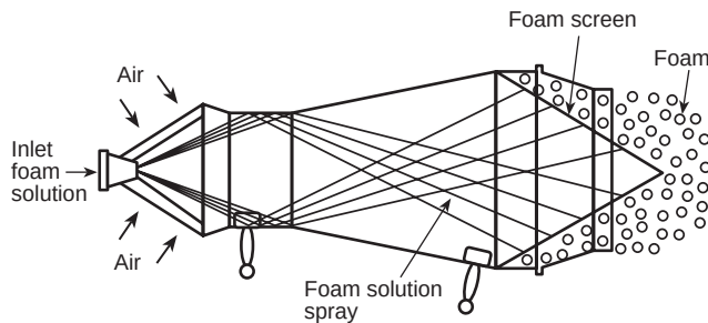
Figure A-1-9.5(a) Aspirating-type foam generator.
