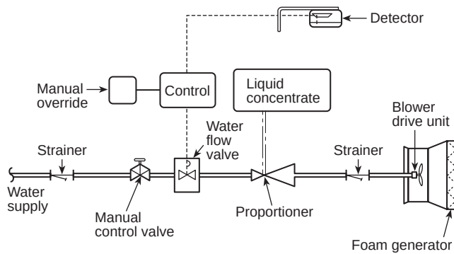
Figure A-1-9.5 Block diagram of automatic medium- or high-expansion foam system.
