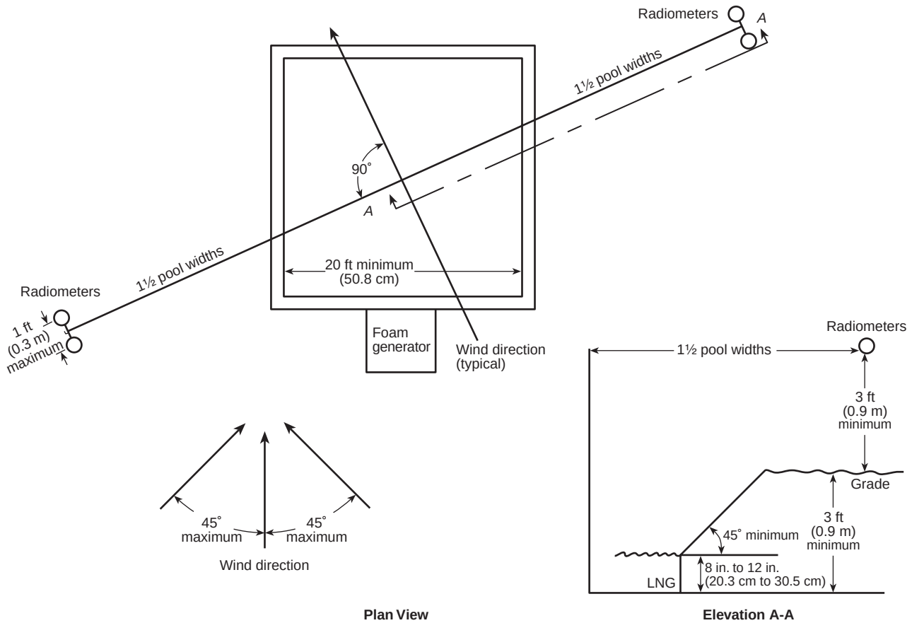
Figure A-1-10.5(d) High-expansion foam standard evaluation test pit.
