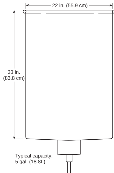
Figure A-1-10.5(b)(2) Typical drainage drum for high-expansion foam expansion and drainage test.
