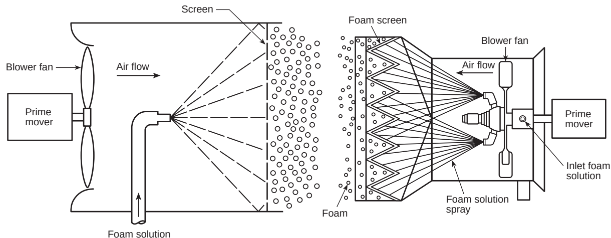
Figure A-1-9.5(b) Blower-type foam generators.
