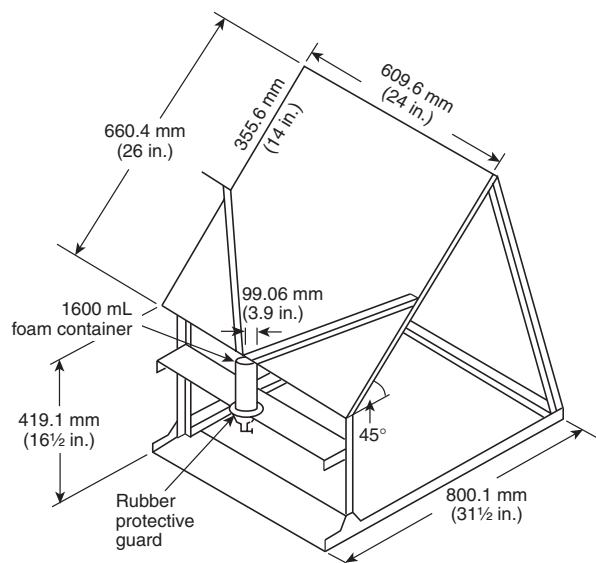
FIGURE D.1.1(a) Foam Sample Collector.
