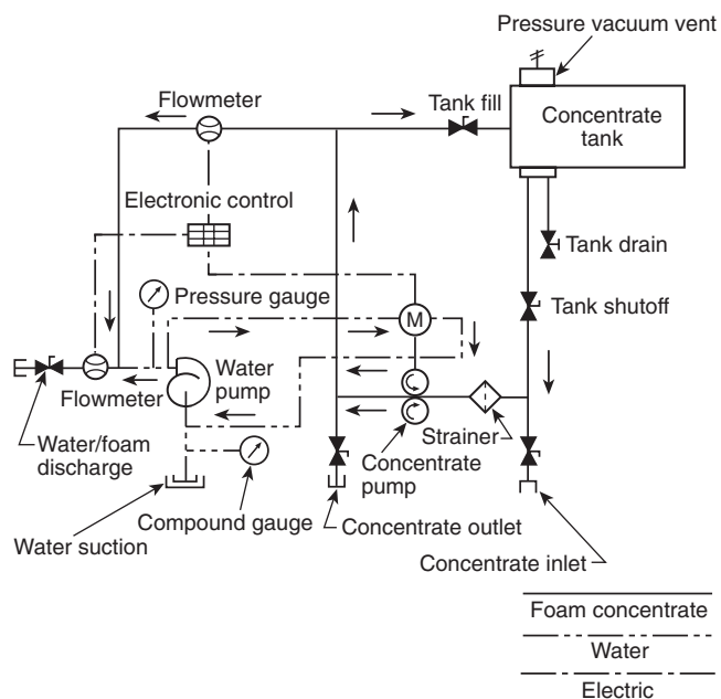
FIGURE A.3.3.23.2(d) Water Turbine-Driven Flow-Sensing Direct Injection Foam Proportioning System.
