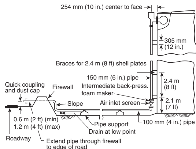
FIGURE A.3.3.5.2(b) Typical Air Foam Piping for Intermediate Back-Pressure Foam System.
