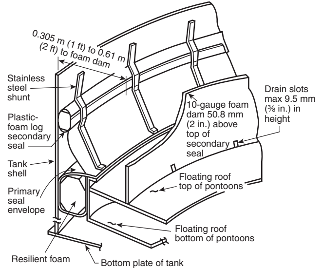
FIGURE 5.3(d) Double Seal System for Floating Roofs Using Plastic-Foam Log (Secondary Seal).
