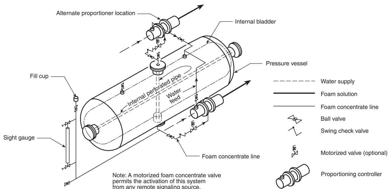
FIGURE A.3.3.27.2(b) Diaphragm (Bladder) Proportioning Tank.
