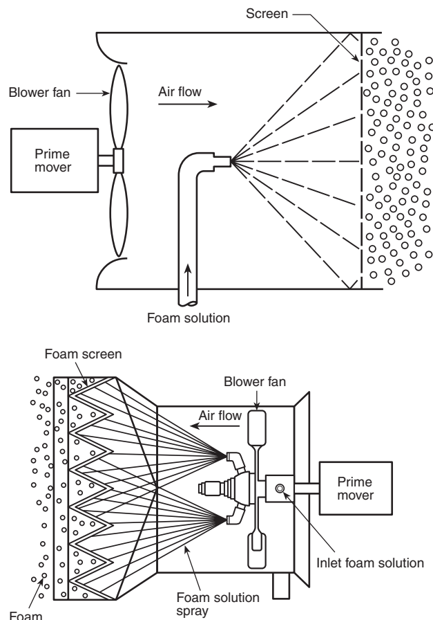
FIGURE A.6.7.4(c) Blower-Type Foam Generators.
