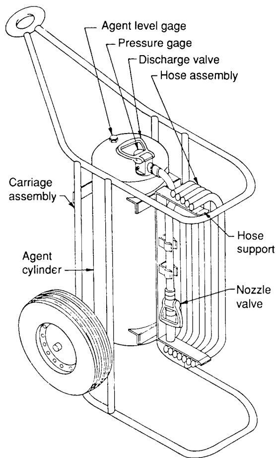
Figure C-3-7(b) Stored Pressure Halon 1211 Type.
