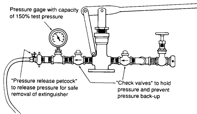
Figure A-5-4.3(a) Hydrostatic Hand Pump.
