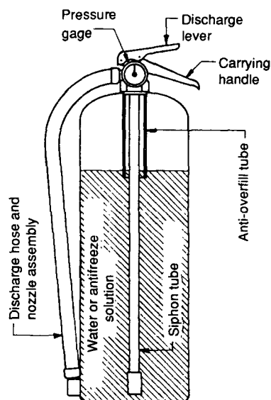
Figure D-4-1.1 Stored Pressure Water Extinguisher.
