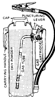
Figure D-4-6.1(a) Cartridge-Operated Dry Powder Extinguisher.
