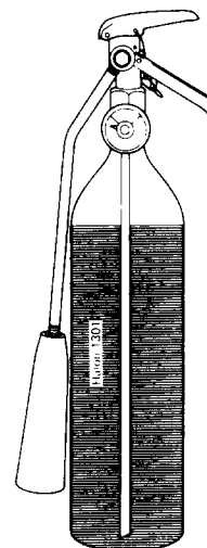
Figure D-4-4.2 Halon 1301 Stored Pressure Fire Extinguisher.
