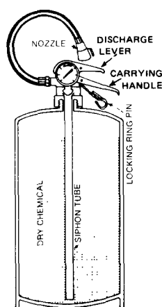
Figure D-4-5(a) Stored Pressure Dry Chemical Extinguisher.
