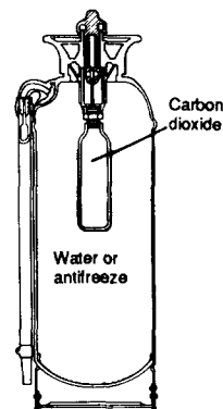
Figure D-4-1.6 Cartridge-Operated Water Fire Extinguisher.
