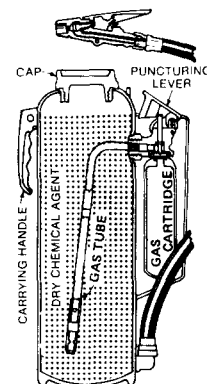
Figure D-4-5(b) Cartridge-Operated Dry Chemical Extinguisher.
