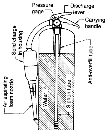
Figure D-4-2.1(b) Stored Pressure AFFF Solid Charge Extinguisher.
