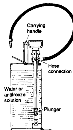
Figure D-4-1.3 Pump Tank Fire Extinguisher.
