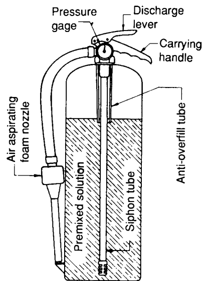
Figure D-4-2.1(a) Stored Pressure AFFF or FFFP Liquid Extinguisher.
