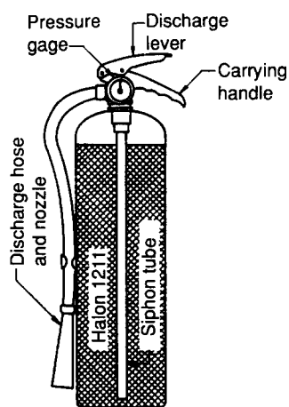
Figure D-4-4.1 Halon 1211 Stored Pressure Fire Extinguisher.
