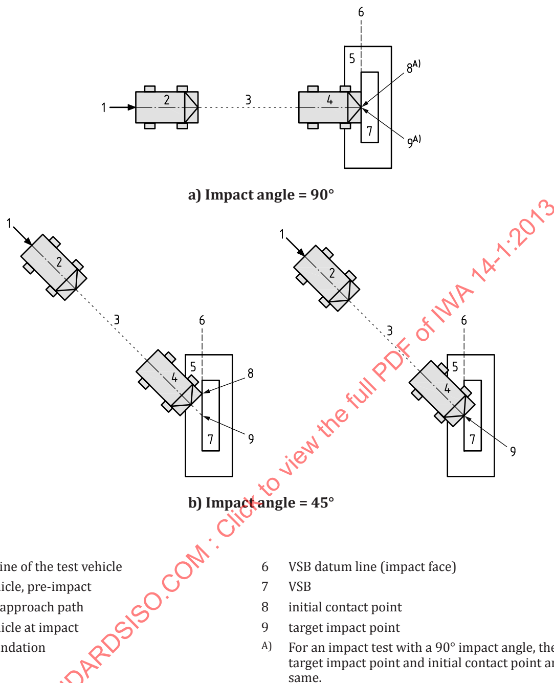
Figure 4 — Impact angle, target impact point and initial contact point — Aerial view
