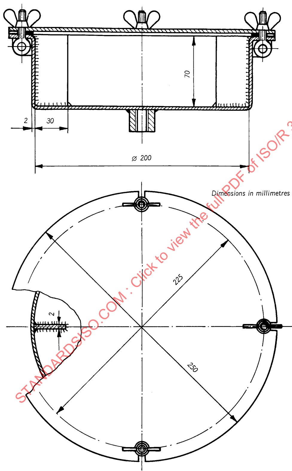
FIG. 2. — Drum used for abrasion test
