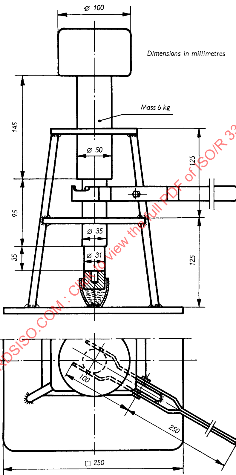
FIG. 1. — Press used for compressing the mixture of anthracite and test coal.
