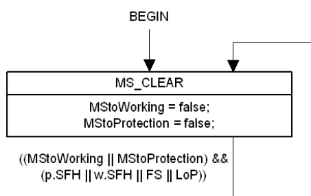
Figure 26-16—Clear Manual Switch state machine
