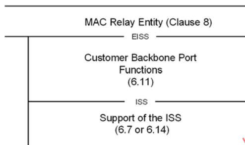
Figure 6-3—B-Component CBP
