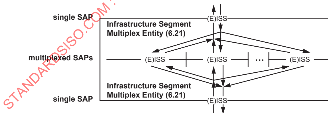
Figure 6-11—Two back-to-back Up and Down Infrastructure Segment Multiplex Entities
