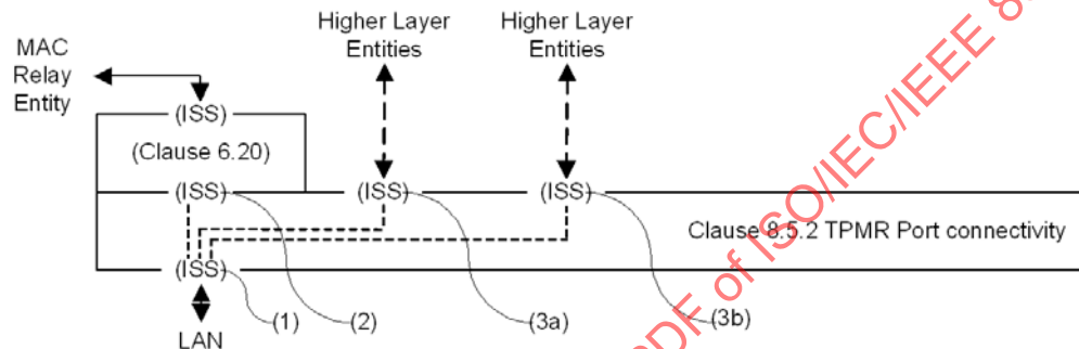
Figure 8-10—TPMR Port Transmit and Receive
