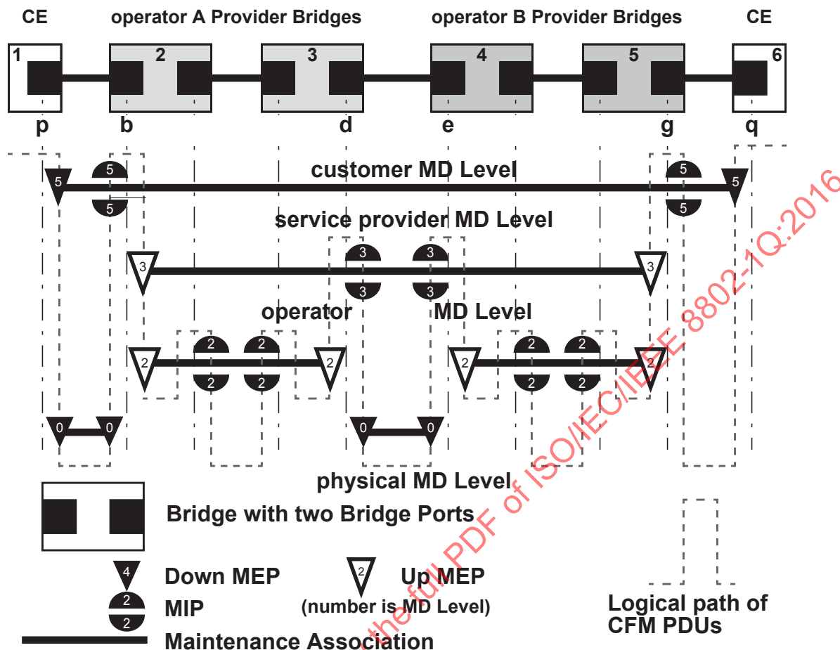
Figure 18-7—MEPs, MIPs, and MD Levels
