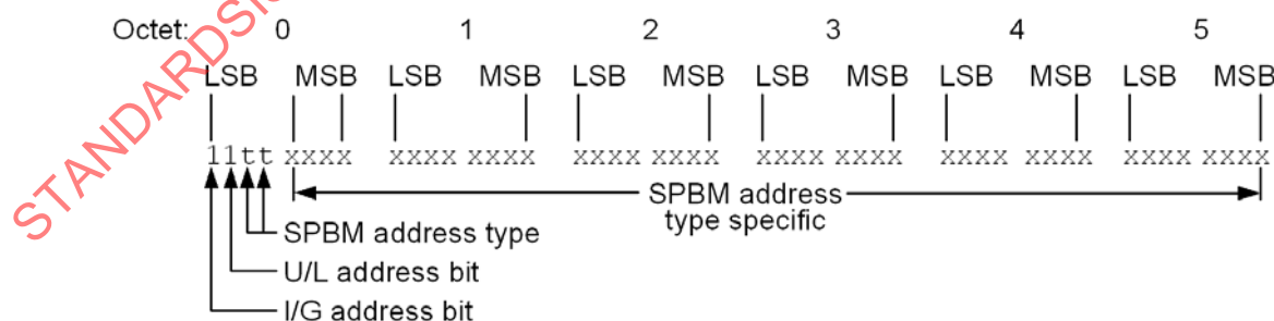
Figure 27-2—SPBM group MAC address—general format
