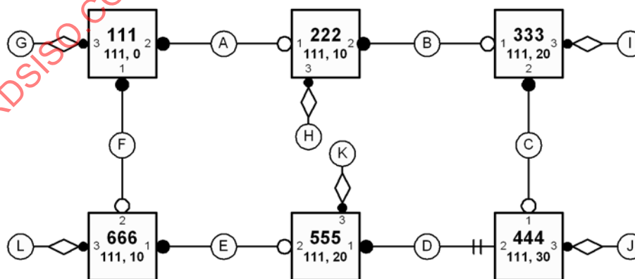
Figure 13-5—“Ring Backbone” example
