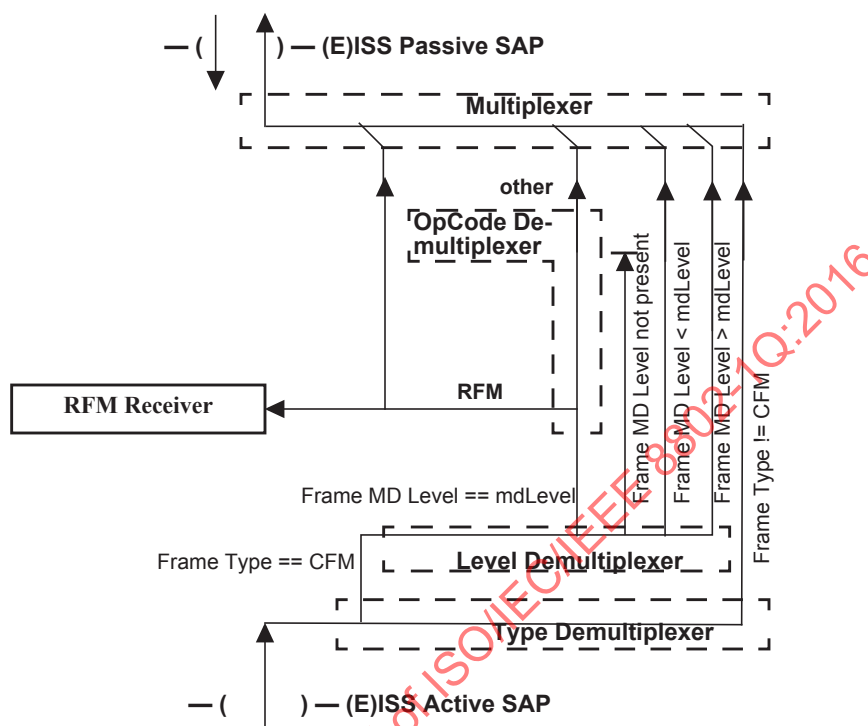
Figure 29-5—RFM Receiver on a non-MP
