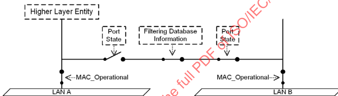
Figure 8-16—Single point of attachment—relay not permitted
