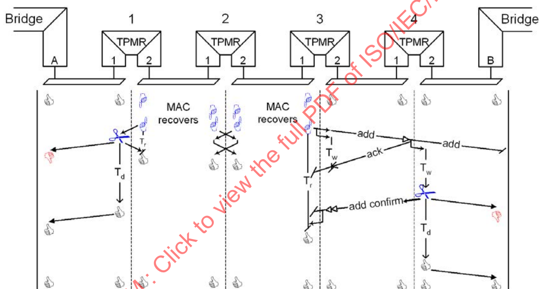
Figure 23-6—TPMR recovery
