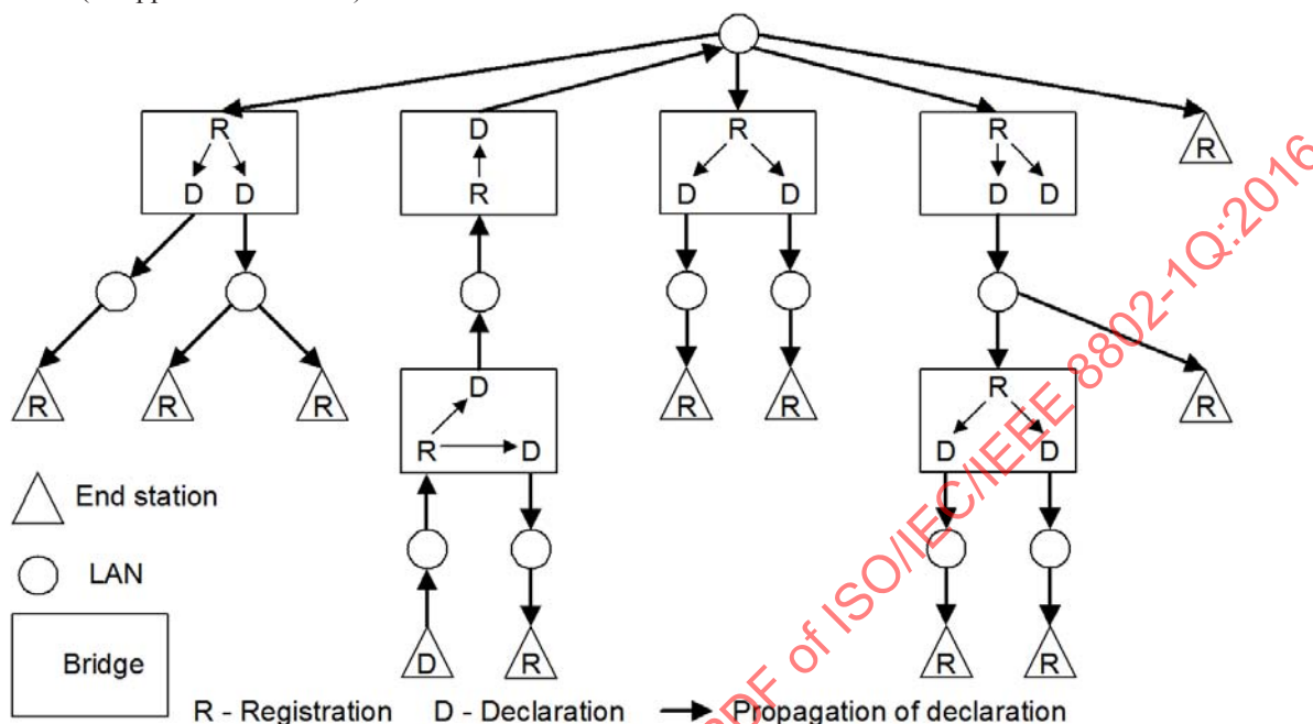
Figure 10-1—Example—Attribute value propagation from one station
