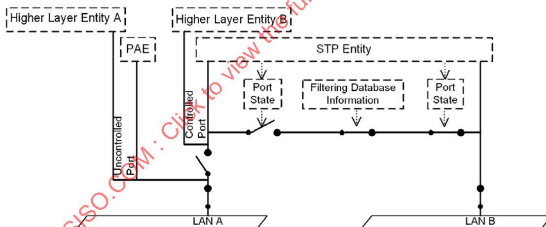
Figure 8-18—Controlled and Uncontrolled Port connectivity
