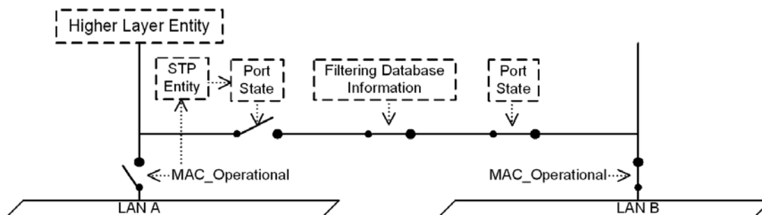
Figure 8-17—Effect of Port State
