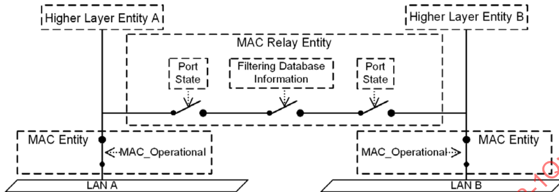
Figure 8-13—Effect of control information on the forwarding path
