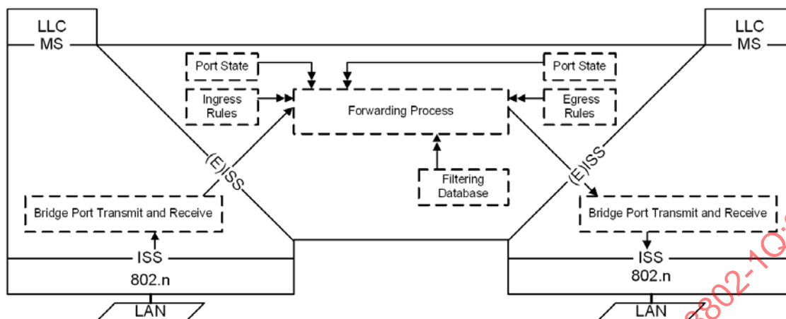
Figure 8-4—Relaying MAC frames
