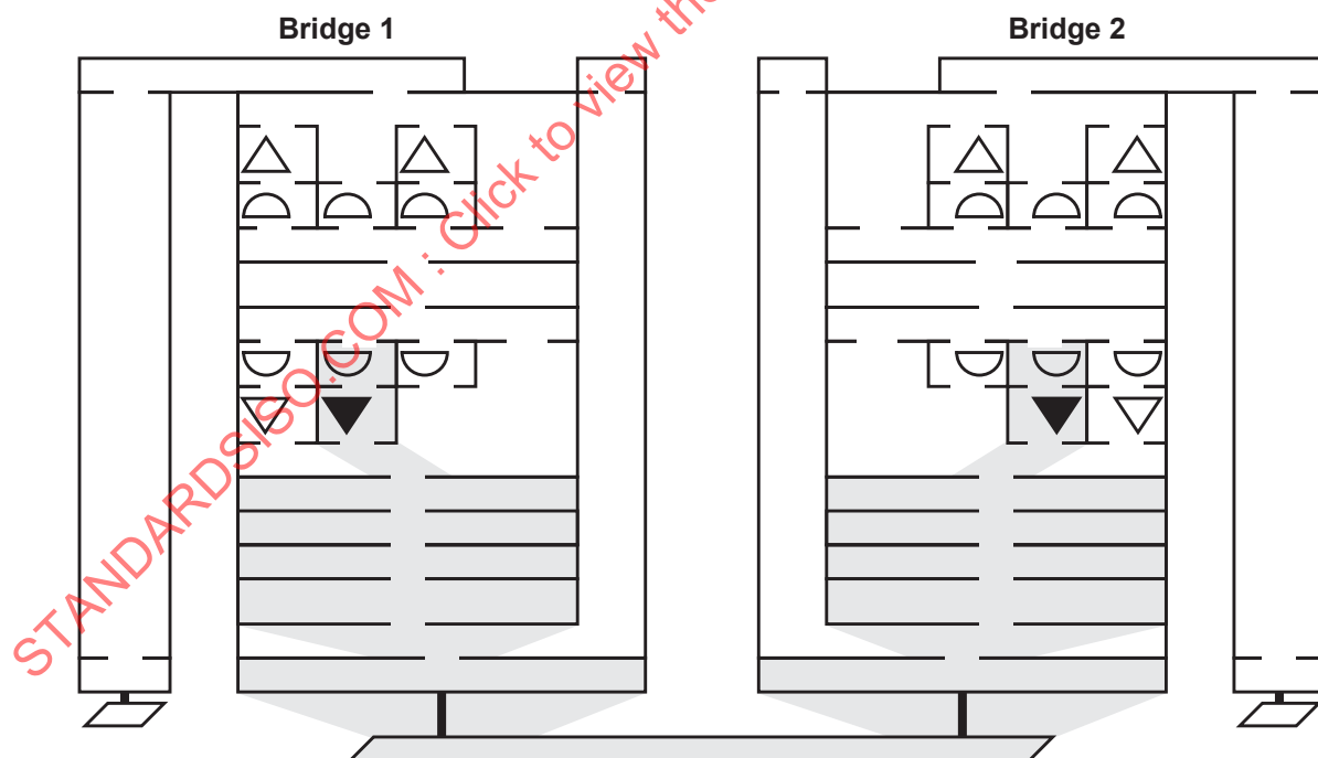
Figure 22-6—Service instance spanning two Bridges protected by Down MPs
