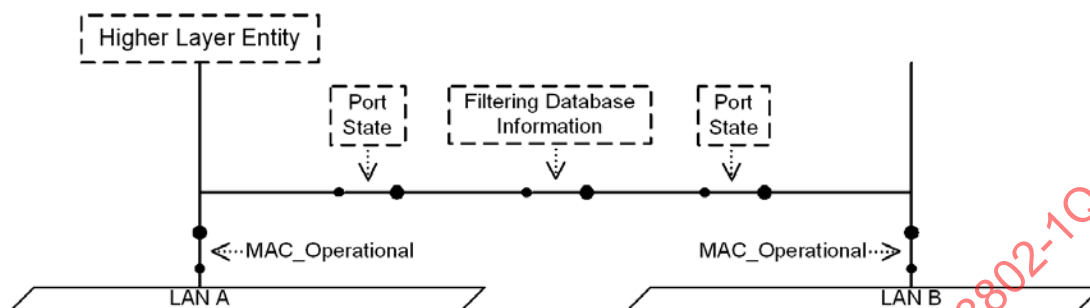
Figure 8-15—Single point of attachment—relay permitted
