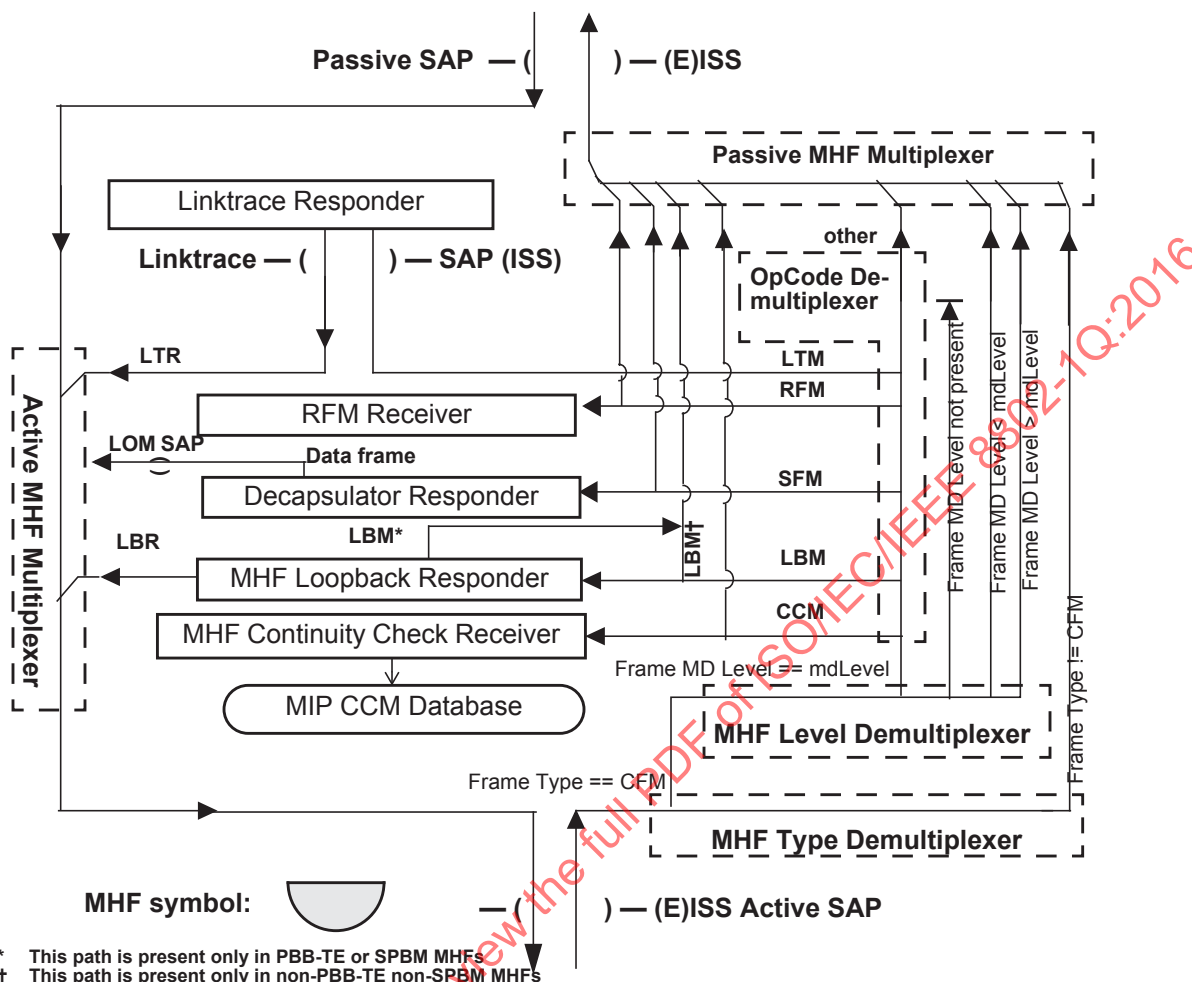
Figure 19-3—MIP Half Function (MHF)
