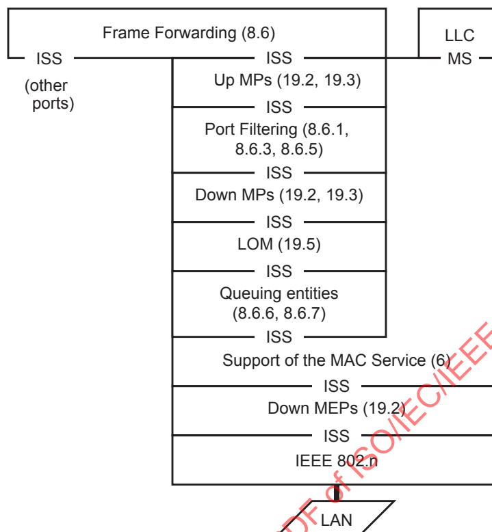
Figure 22-7—MP placement in a non-VLAN aware Bridge Port
