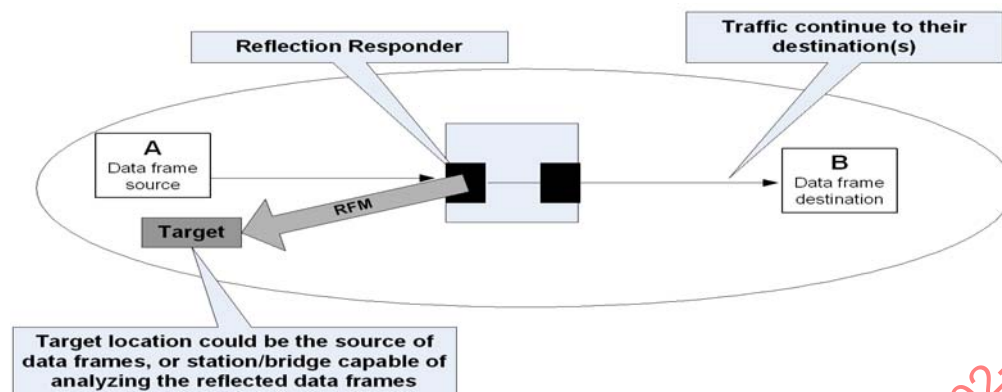
Figure 29-1—Forward path test (FPT)
