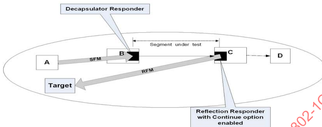
Figure 29-3—Combination of FPT and RPT
