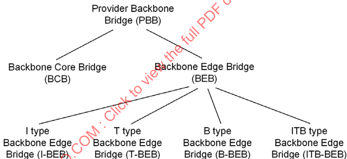
Figure 25-2—PBB terminology
