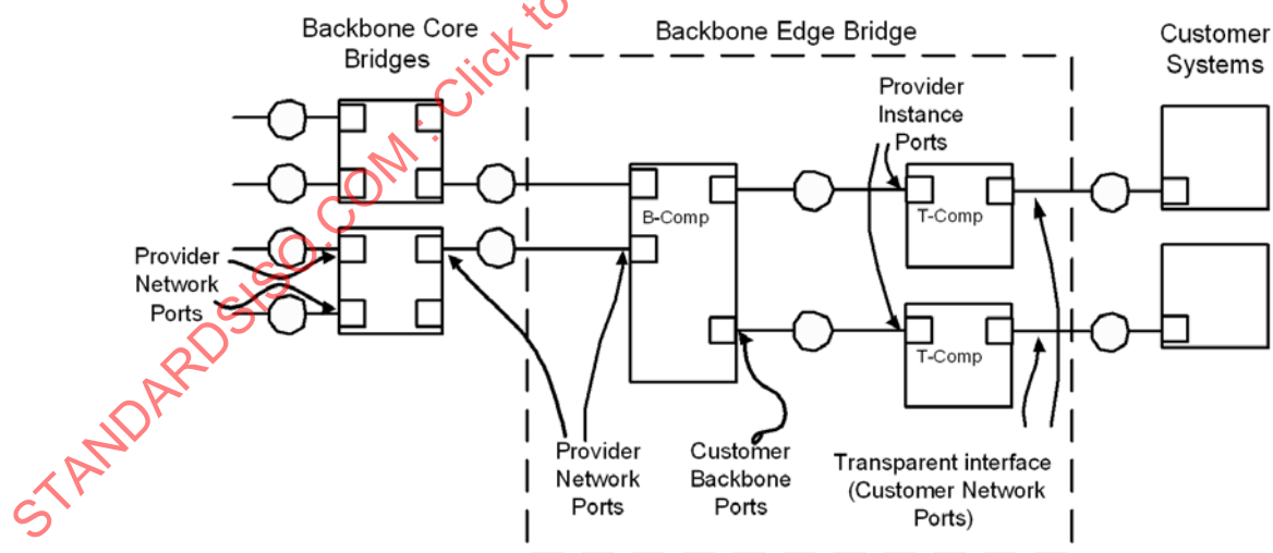
Figure 25-16—Transparent service interface equipment
