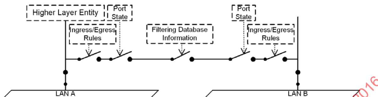
Figure 8-19—Ingress/egress control information in the forwarding path
