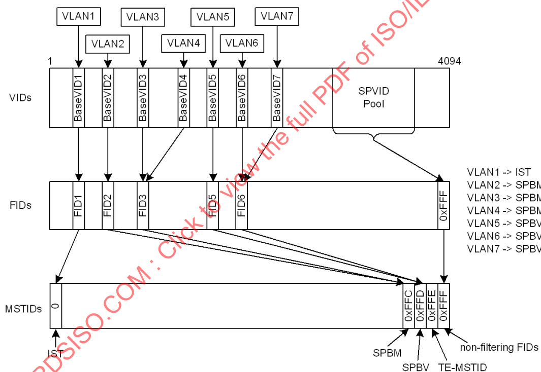
Figure 27-1—Configuring VLAN support in an SPT Region (example)
