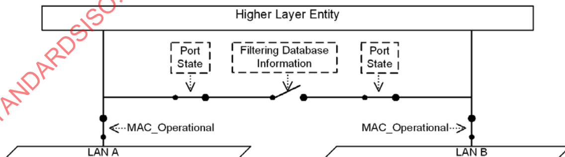
Figure 8-14—Per-Port points of attachment
