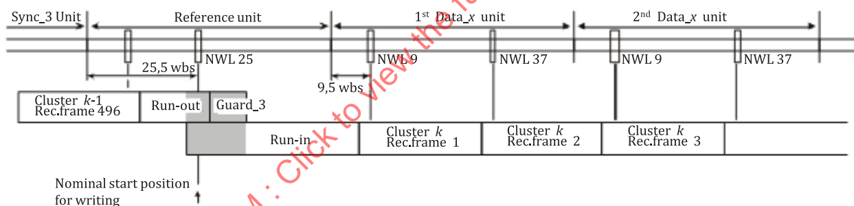
Figure 51 — Example of nominal start position for data recording
