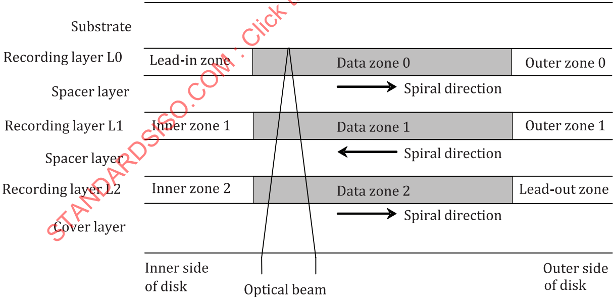
Figure 14 — Subdivision of information zone
