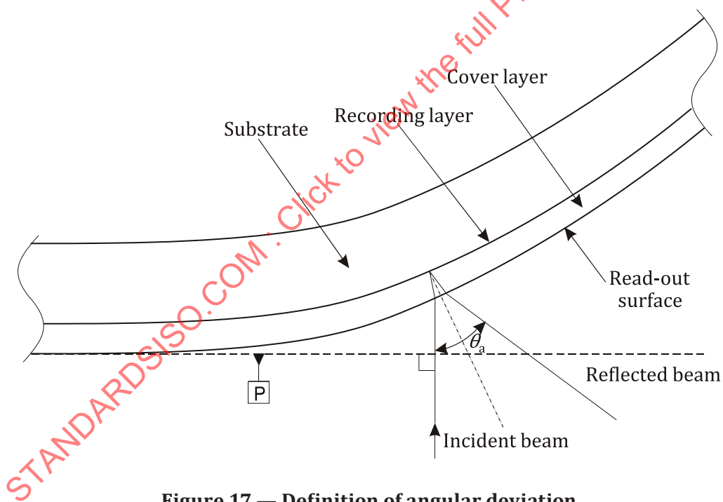
Figure 17 — Definition of angular deviation
