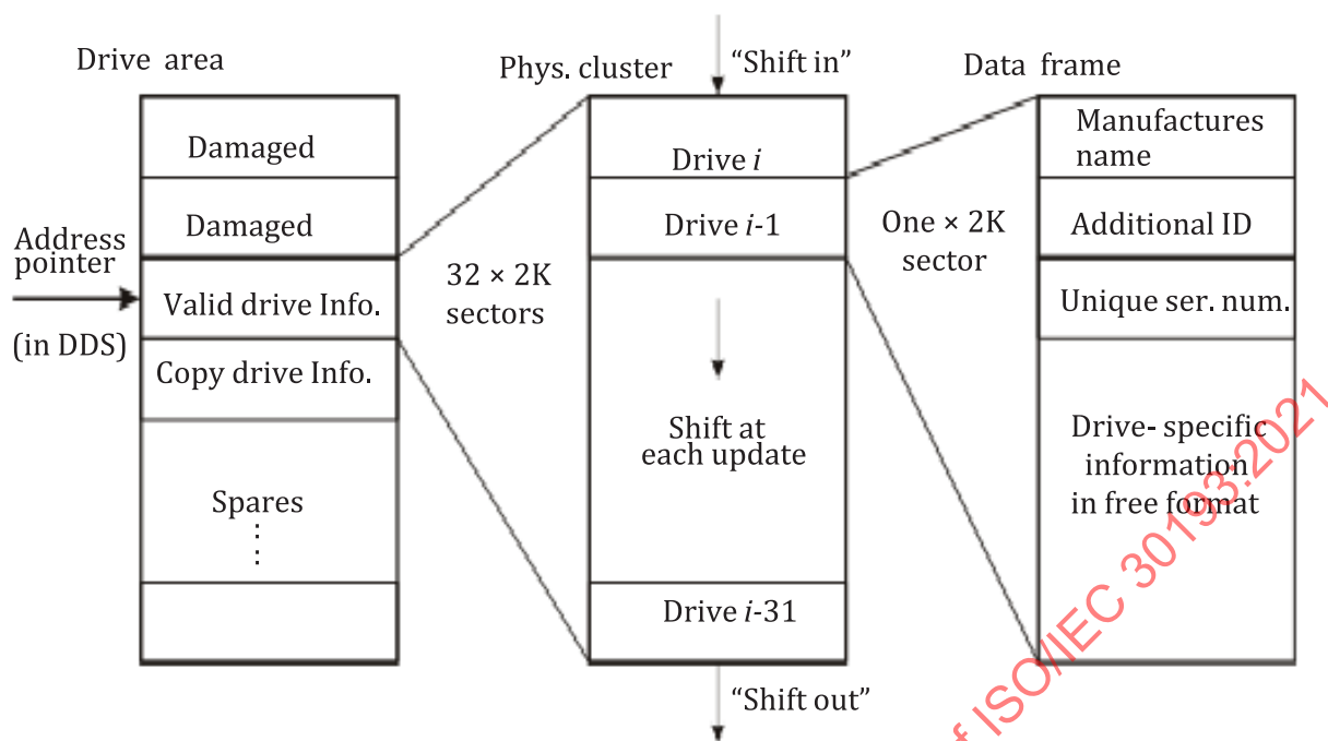
Figure 97 — Format of drive area (example)
