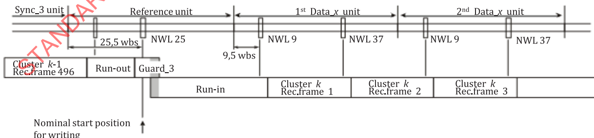
Figure 52 — Example of data recording with maximum overlap
