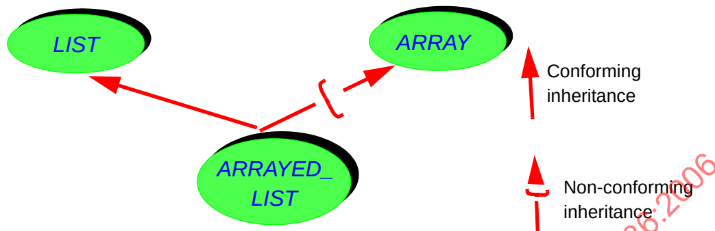
Figure 3: Inheritance
