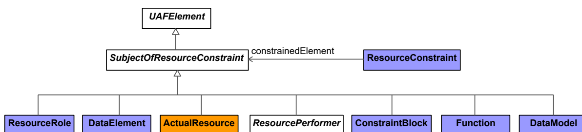
Figure 9:134 - SubjectOfResourceConstraint
