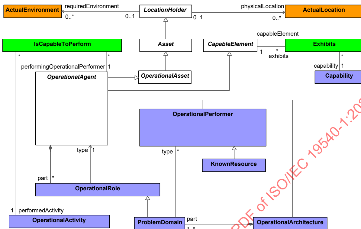
Figure 8:10 - Operational Structure
