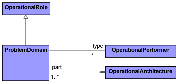
Figure 9:61 - ProblemDomain
