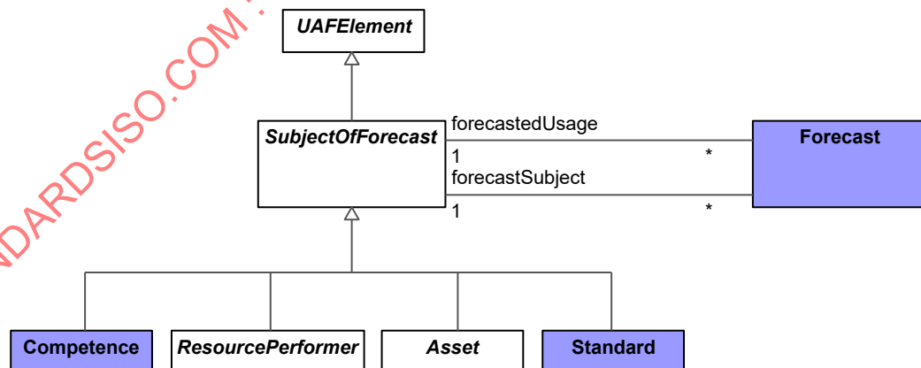
Figure 9:136 - SubjectOfForecast
