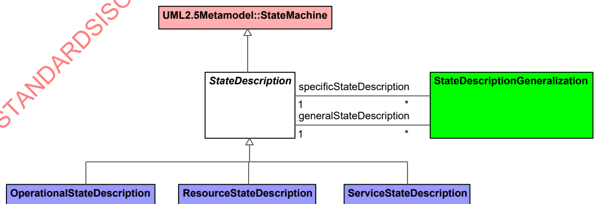
Figure 9:20 - StateDescription
