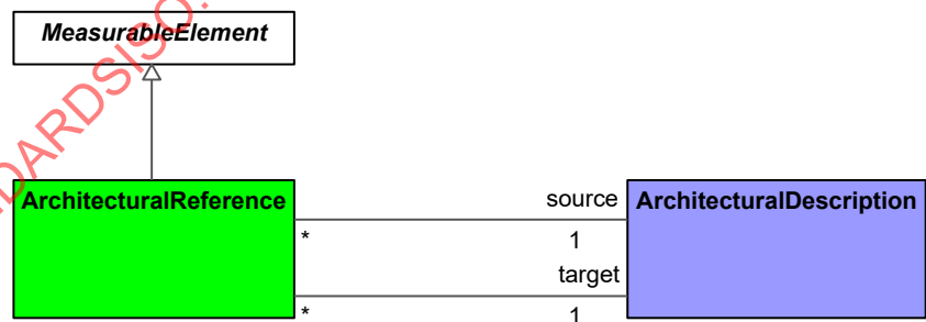
Figure 9:25 - ArchitecturalReference
