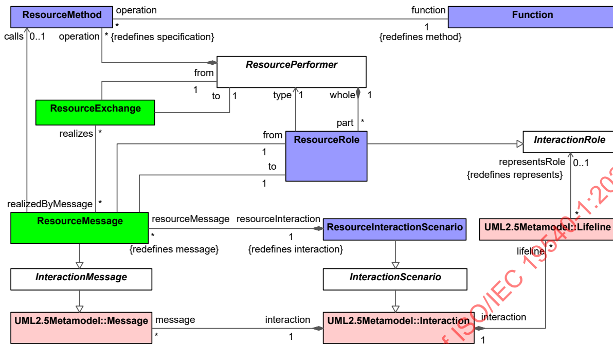
Figure 8:47 - Resources Interaction Scenarios
