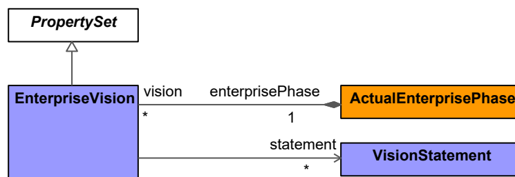
Figure 9:35 - EnterpriseVision
