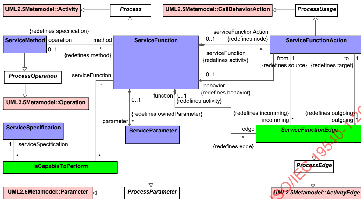
Figure 8:21 - Services Processes
