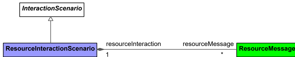
Figure 9:103 - ResourceInteractionScenario
