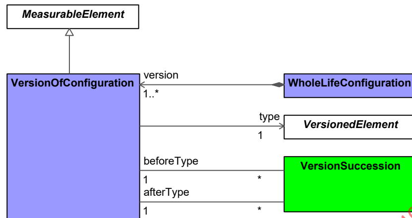
Figure 9:139 - VersionOfConfiguration
