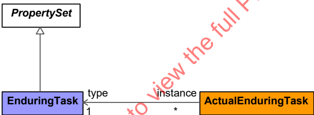
Figure 9:32 - EnduringTask
