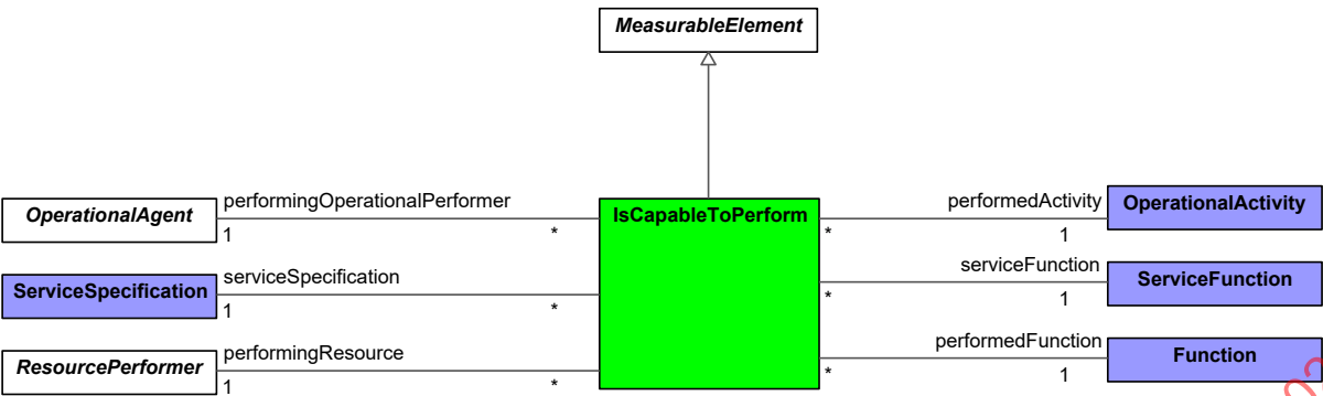
Figure 9:12 - IsCapableToPerform
