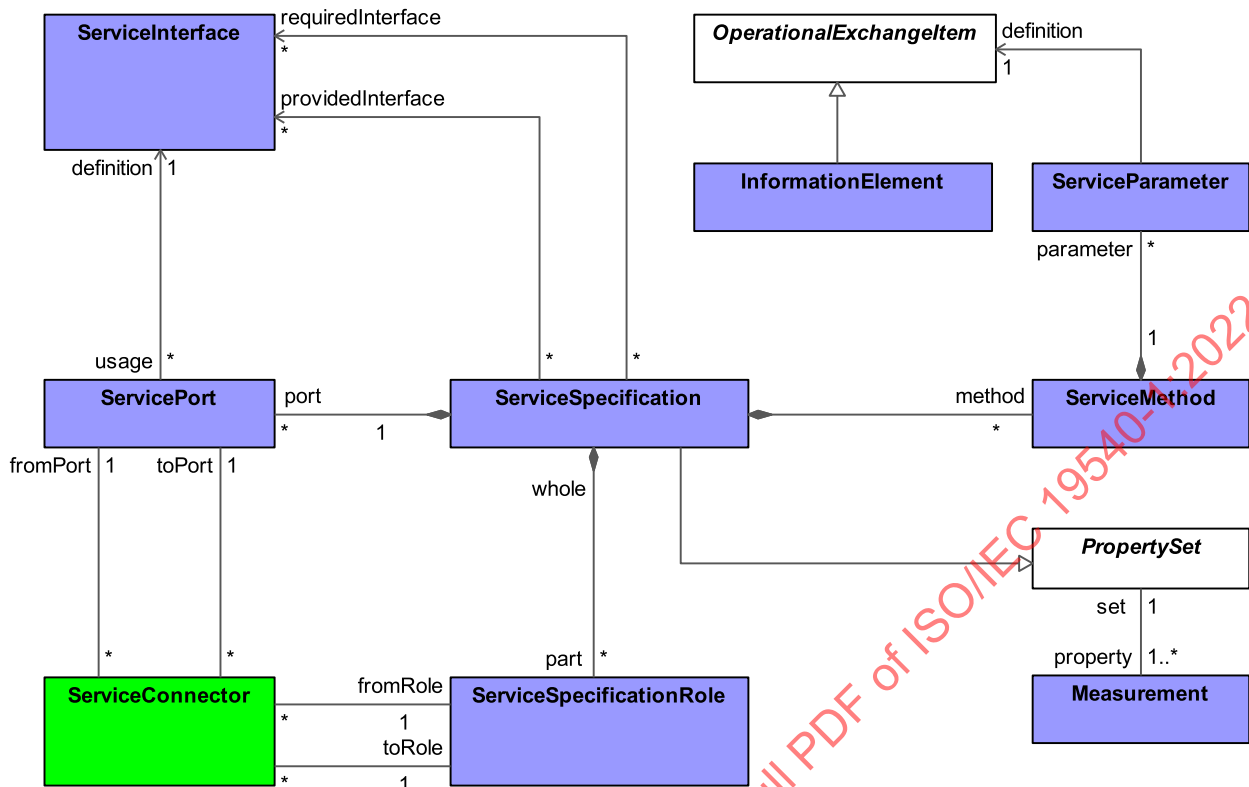
Figure 8:19 - Services Structure
