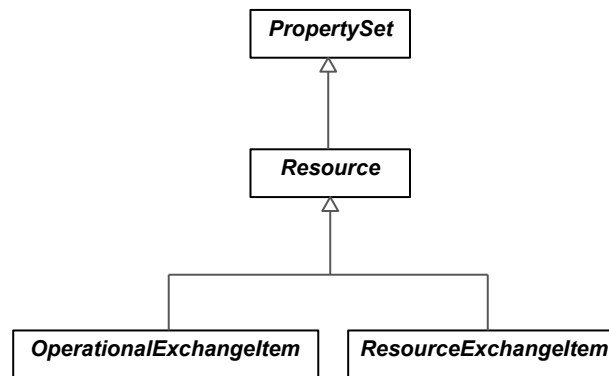
Figure 9:10 - Resource
