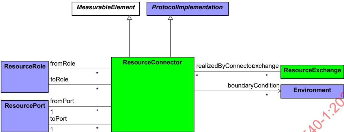
Figure 9:121 - ResourceConnector
