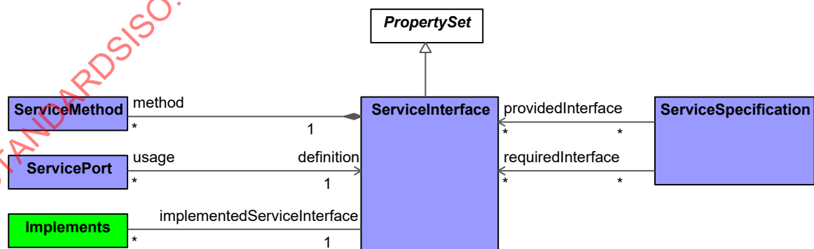
Figure 9:84 - ServiceInterface
