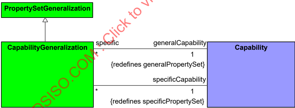
Figure 9:28 - CapabilityGeneralization
