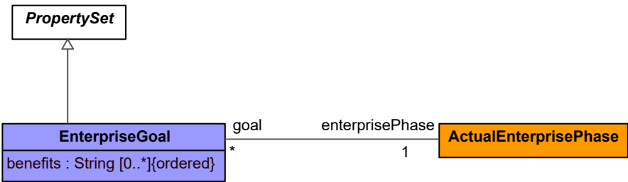
Figure 9:33 - EnterpriseGoal
