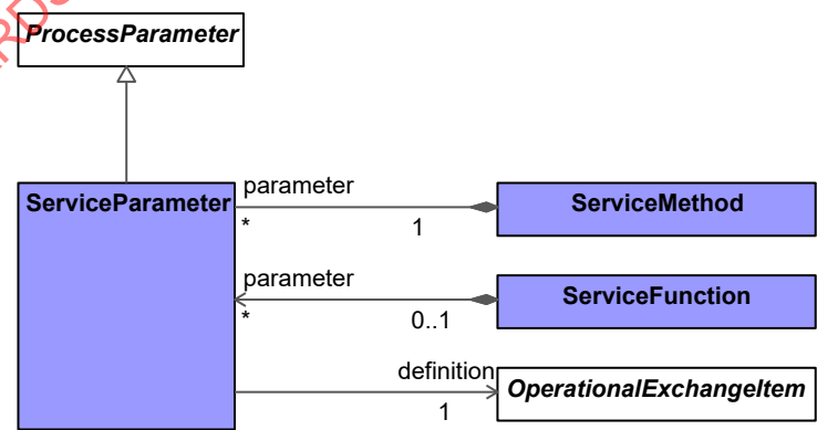
Figure 9:82 - ServiceParameter
