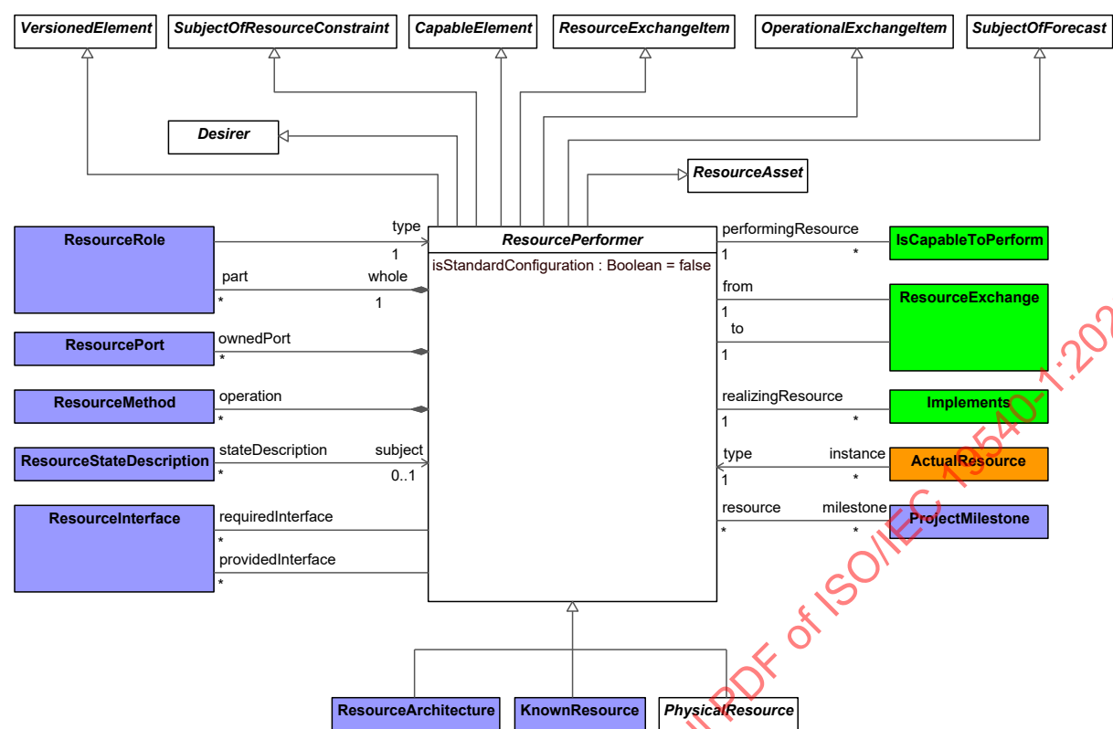
Figure 9:114 – ResourcePerformer
