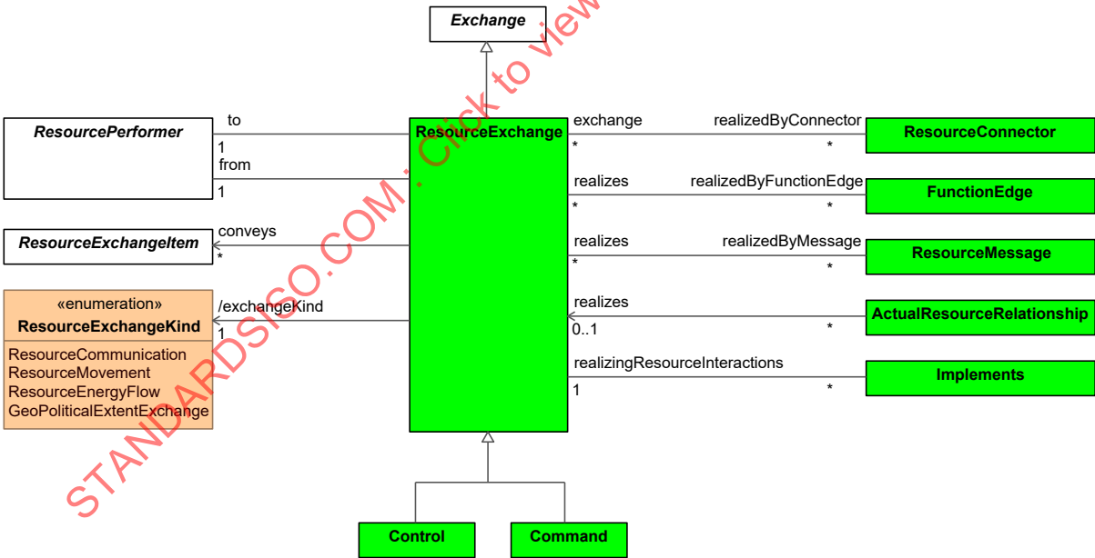
Figure 9:122 - ResourceExchange
