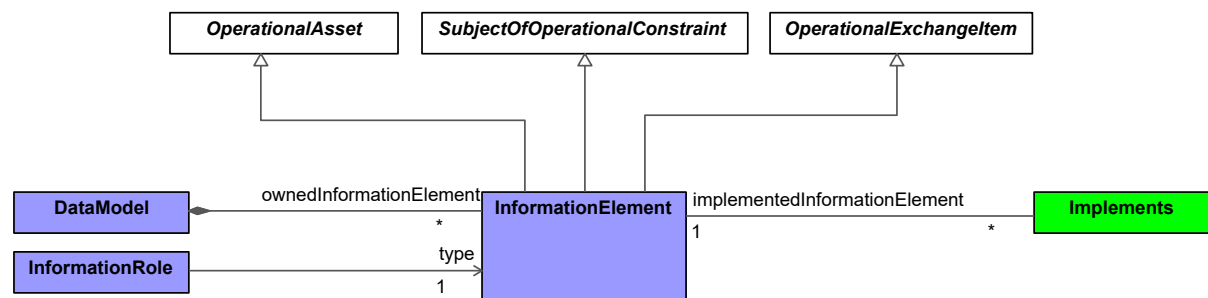
Figure 9:75 - InformationElement
