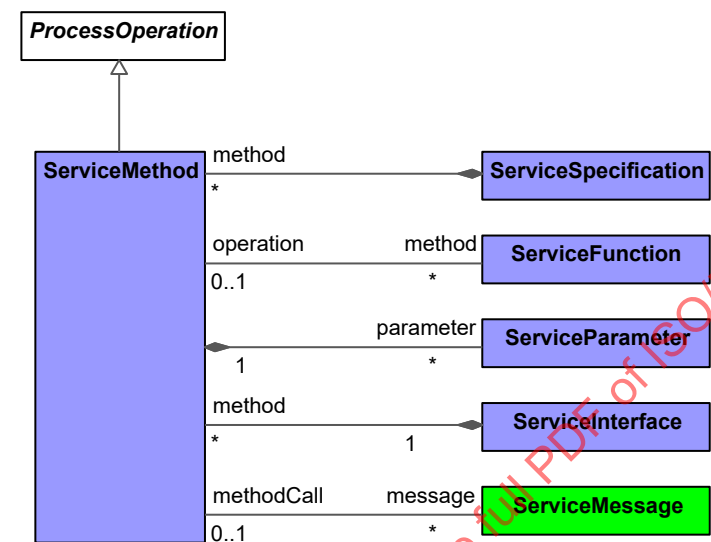
Figure 9:81 - ServiceMethod
