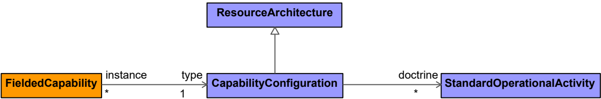
Figure 9:109 - CapabilityConfiguration
