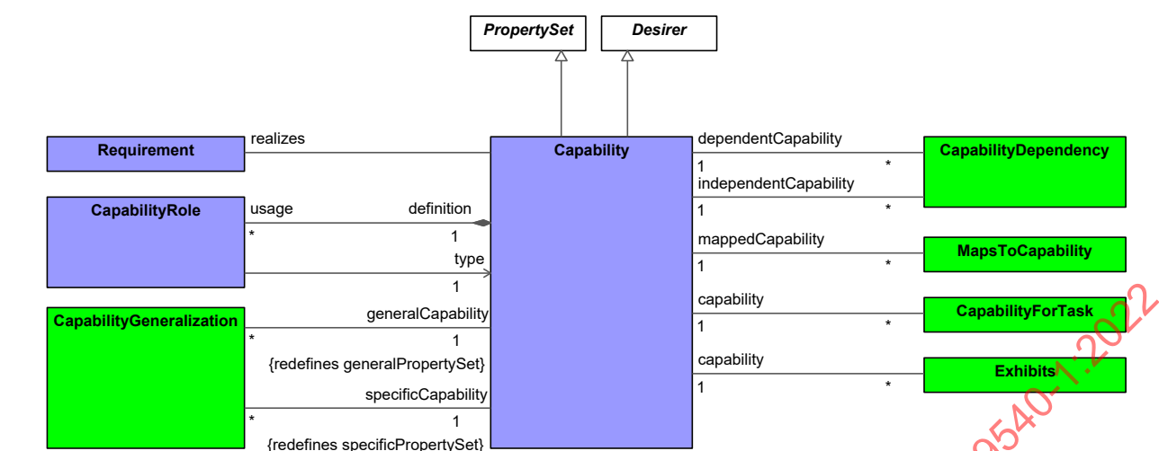
Figure 9:27 - Capability
