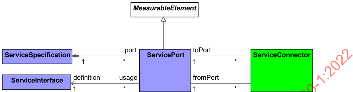
Figure 9:85 - ServicePort
