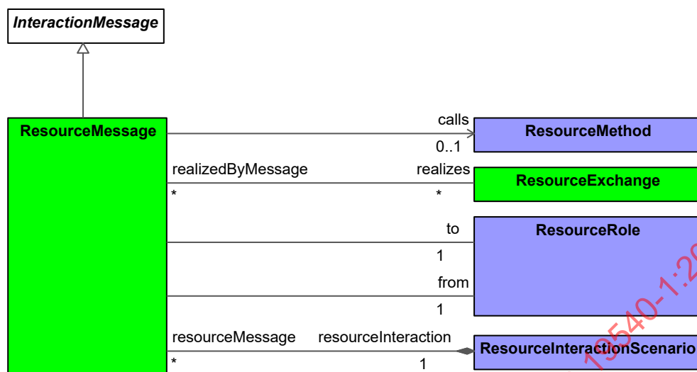
Figure 9:130 - ResourceMessage
