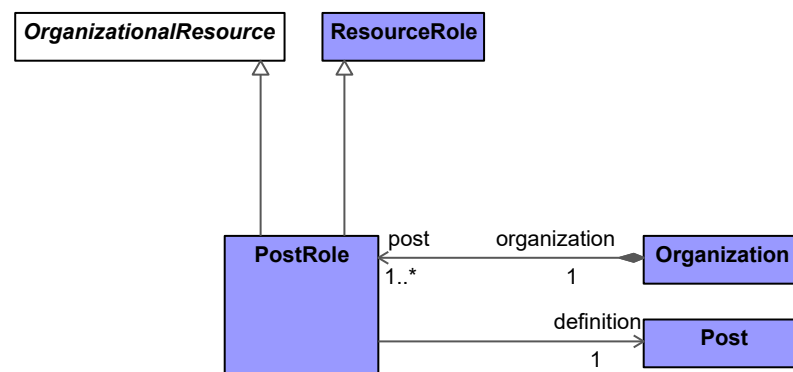
Figure 9:99 - PostRole
