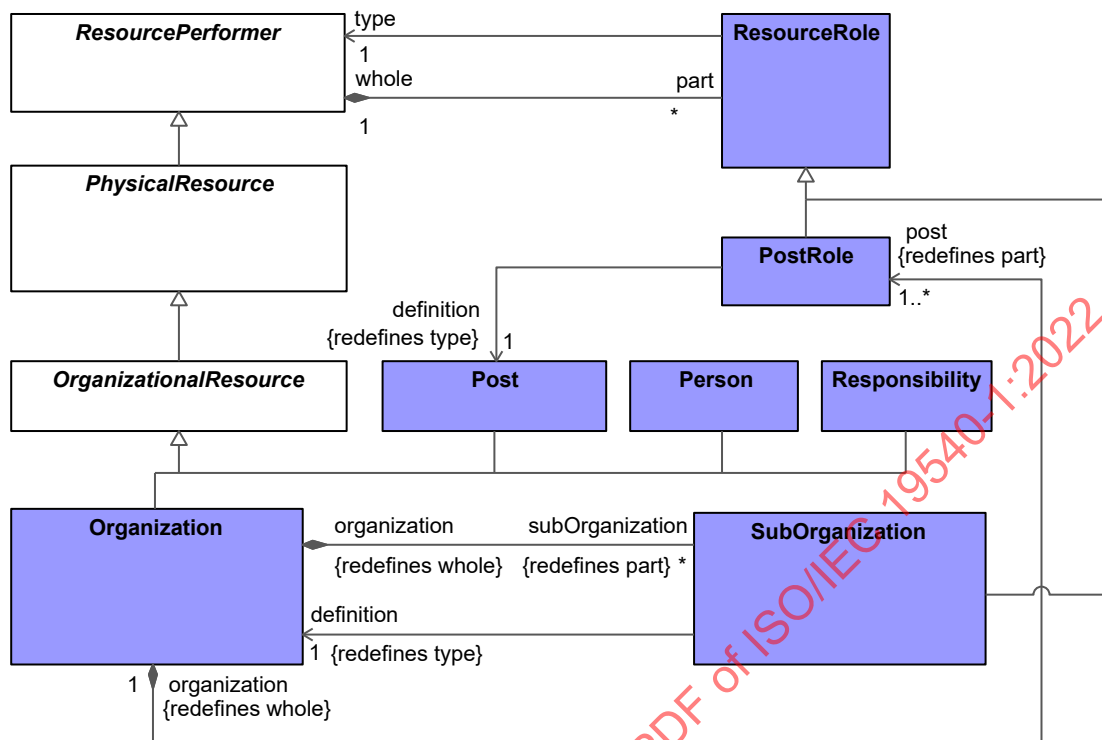
Figure 8:29 - Personnel Structure
