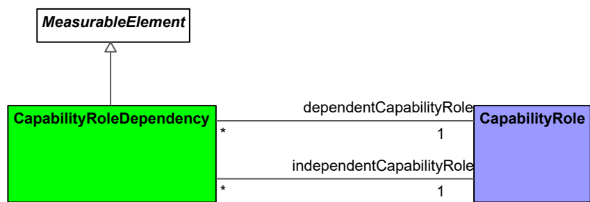
Figure 9:41 - CapabilityRoleDependency
