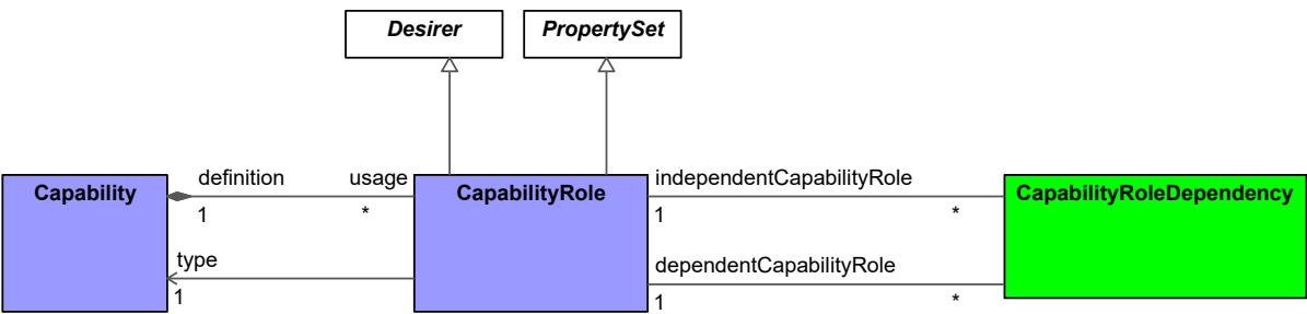
Figure 9:31 - CapabilityRole
