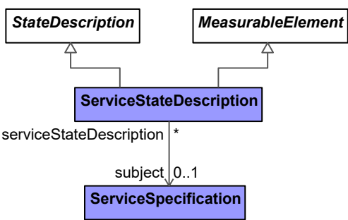
Figure 9:89 - ServiceStateDescription
