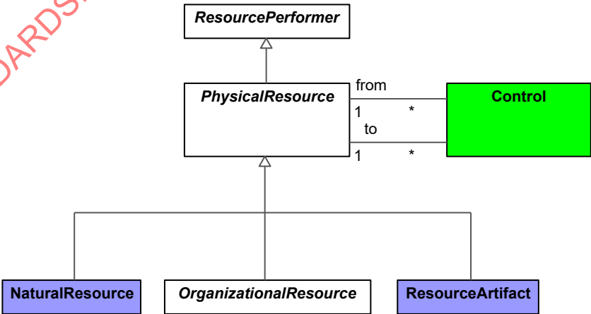
Figure 9:111 - PhysicalResource
