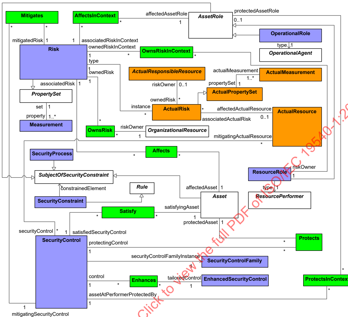
Figure 8:56 - Security Constraints
