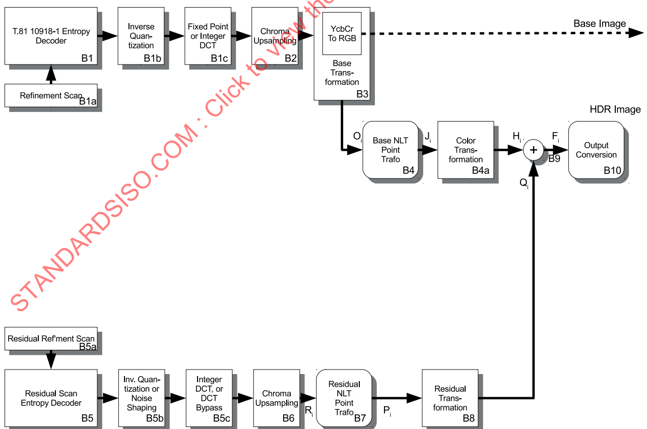
Figure A.1 — High-level overview of the decoding process of a compliant decoder
