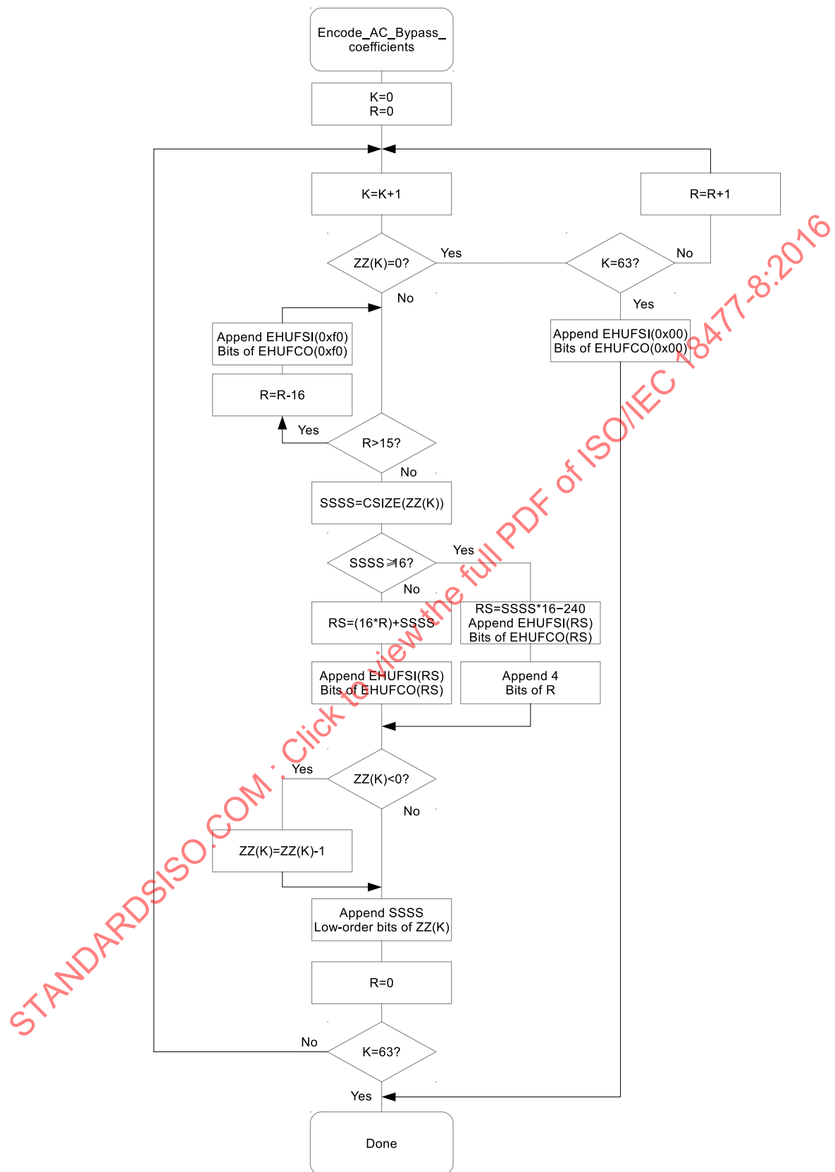
Figure D.3 — Encoding procedure for large-range coding
