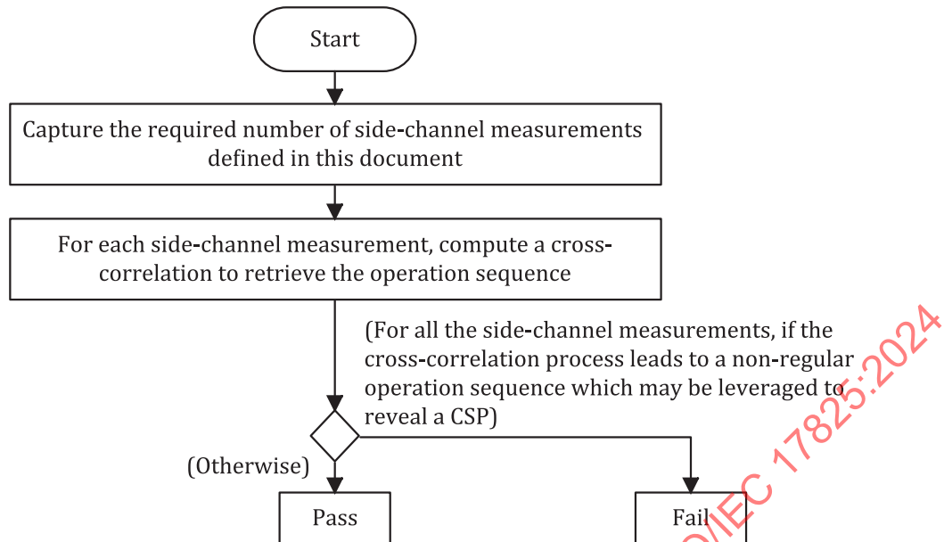
Figure 5 — SPA (SEMA) leakage analysis
