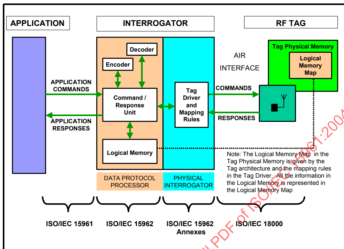
Figure 2 — Logical Functions and Interfaces
