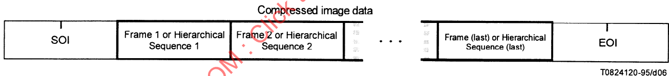
Figure B.6 – Image tiling high level syntax
