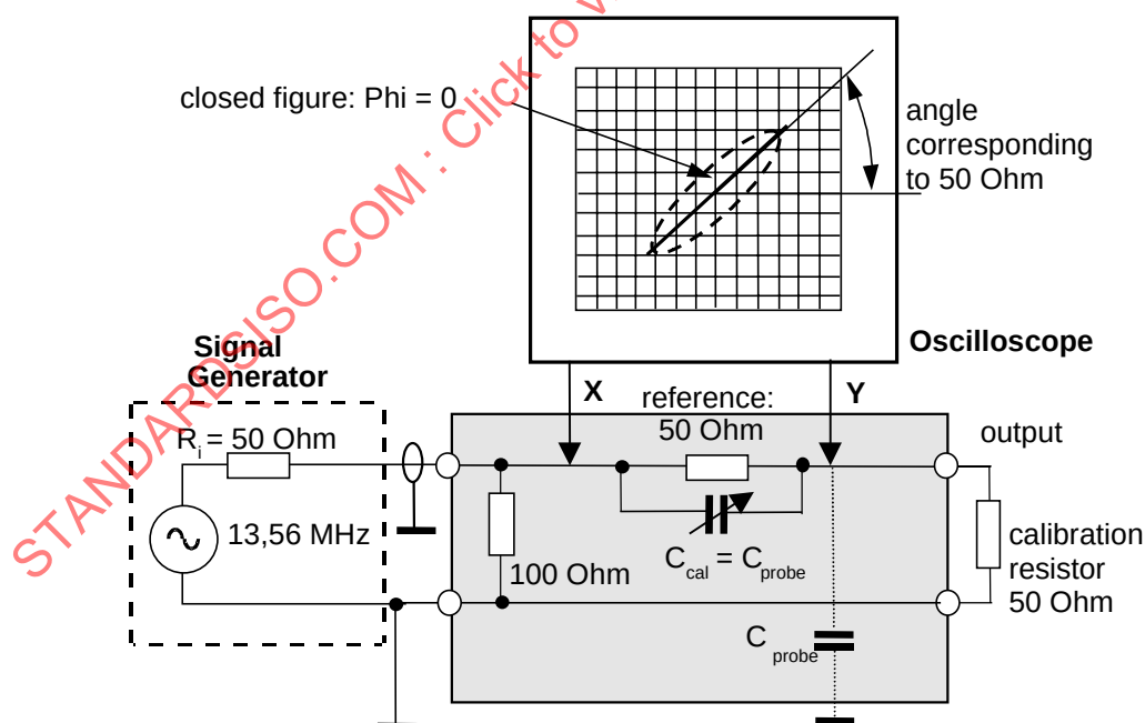
Figure B.1 — Calibration set-up (Step 1)
