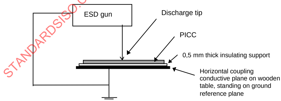
Figure 1 — ESD test circuit
