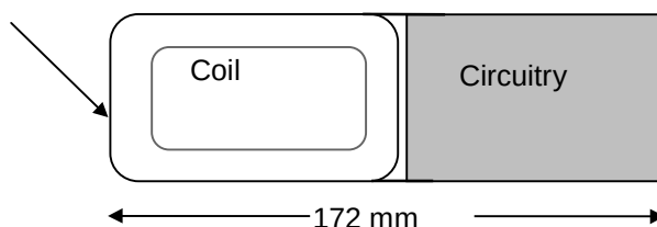
Figure 6 — Reference PICC dimensions
