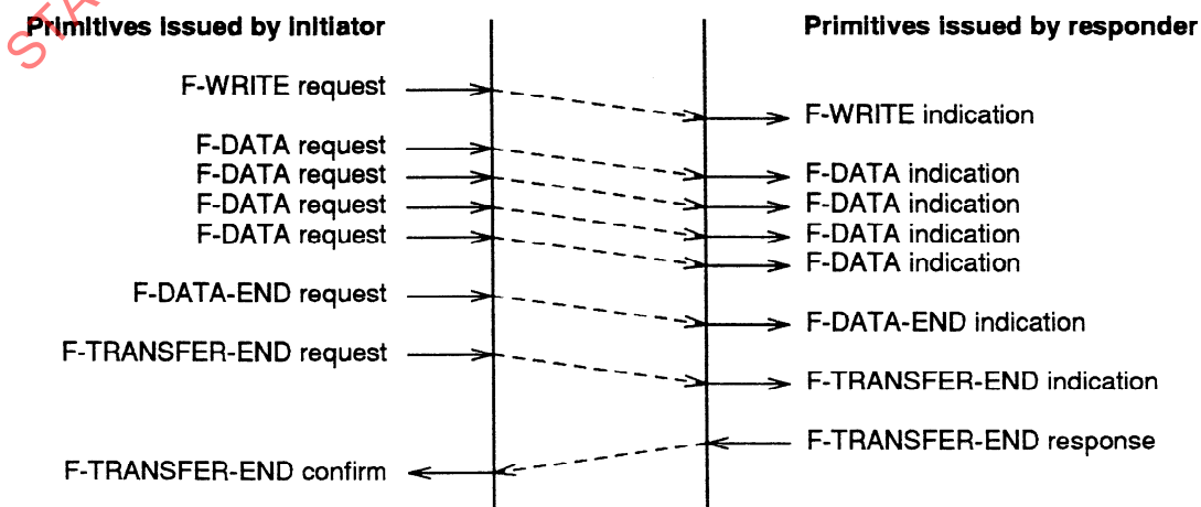
Figure 9 — Sequence of primitives on write
