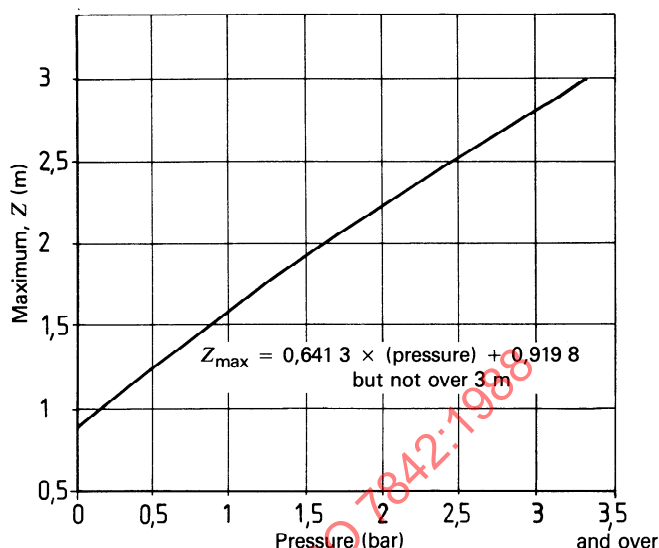
Figure 3 — Maximum submergence on steam trap versus test pressure
