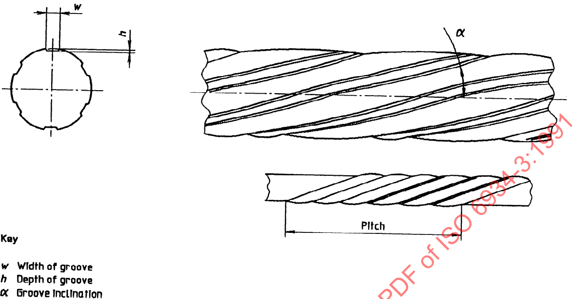
Figure A.2 — Quenched and tempered grooved wire
