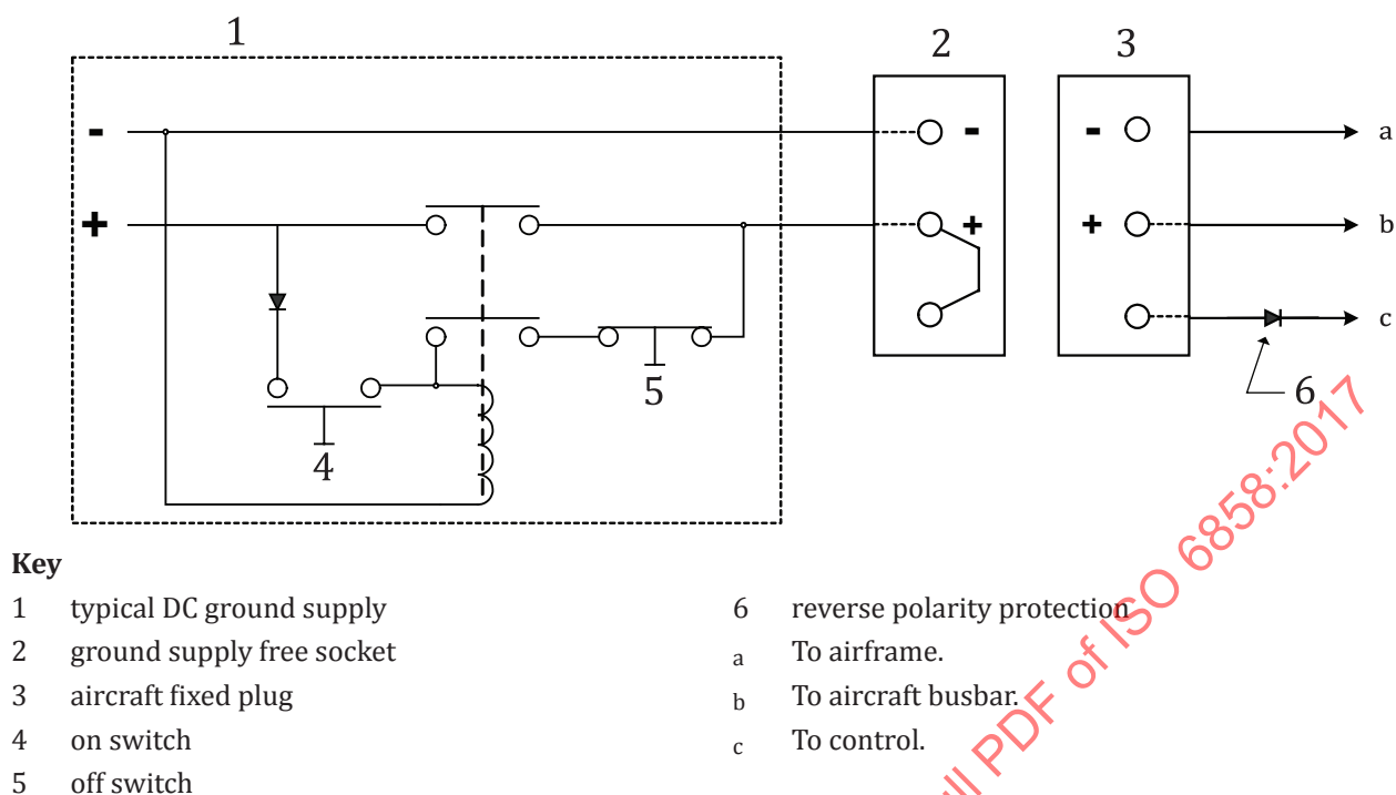
Figure 3 — Standard wiring diagram for DC plug and socket
