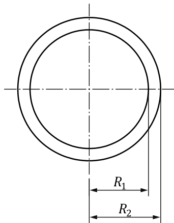
a) Radial clearance, C_R = R_2 - R_1
