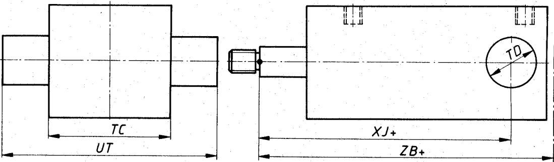
Figure 9 — MT2 — Cap integral trunnion (male) mounting
