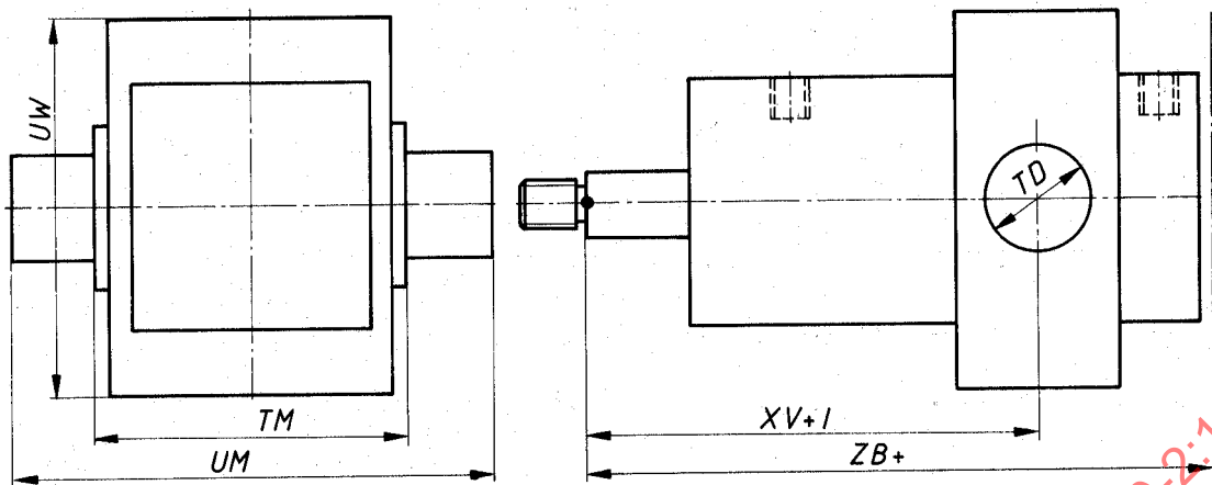
Figure 10 – MT4 – Intermediate fixed or movable trunnion (male) mounting
