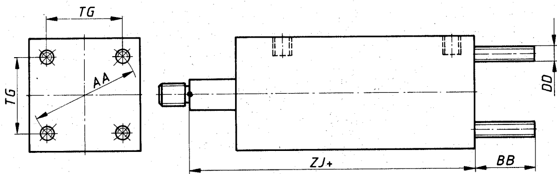
Figure 12 — MX2 — Cap studs or tie rods extended mounting
