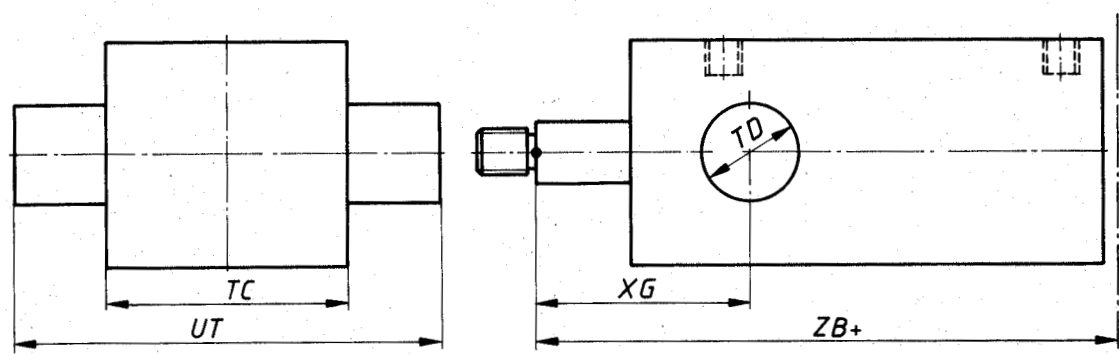
Figure 8 — MT1 — Head integral trunnion (male) mounting
