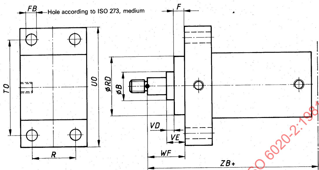
Figure 2 — ME5 — Head rectangular mounting
