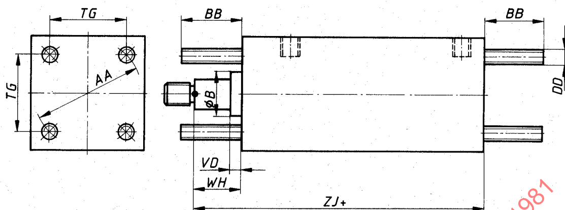
Figure 11 — MX1 — Both ends studs or tie rods extended mounting
