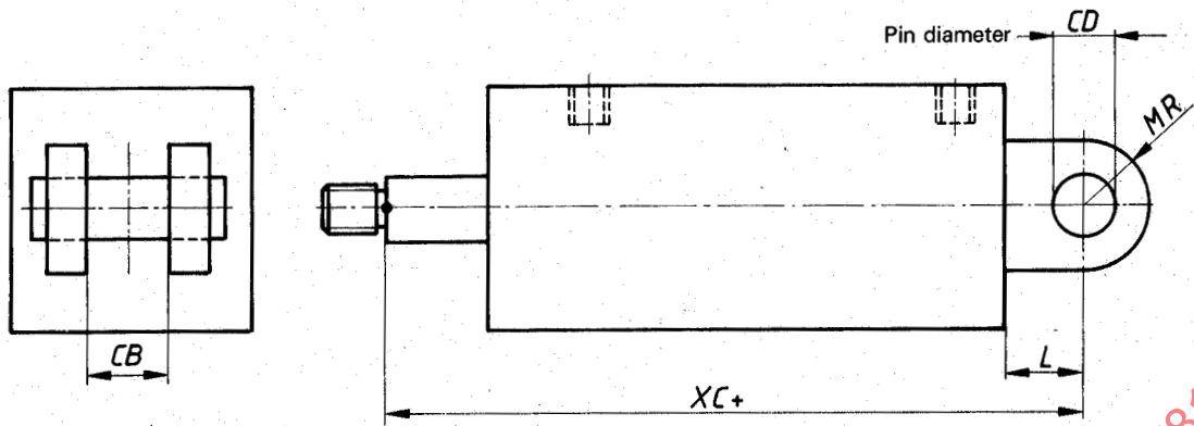
Figure 4 – MP1 – Cap fixed clevis mounting
