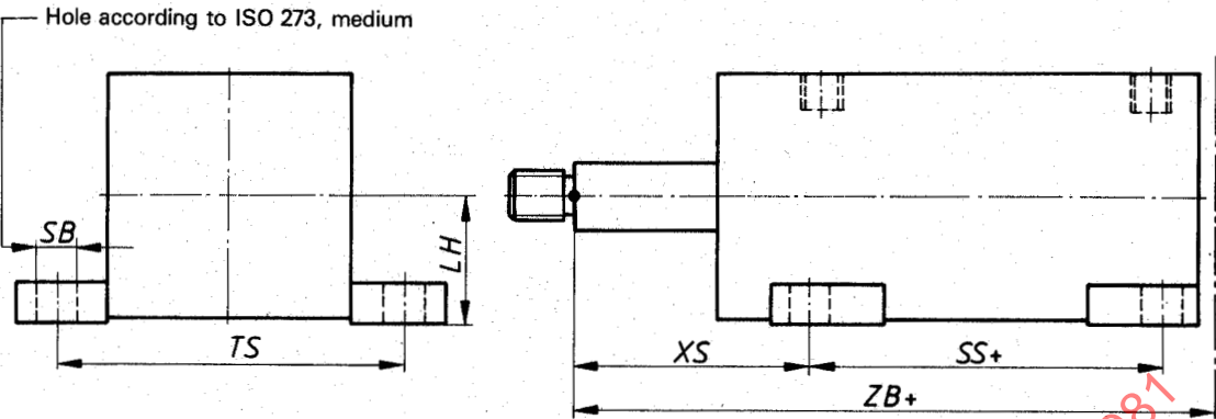
Figure 7 — MS2 — Side lugs mounting
