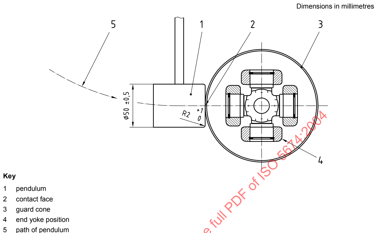
Figure 2 — Impact test
