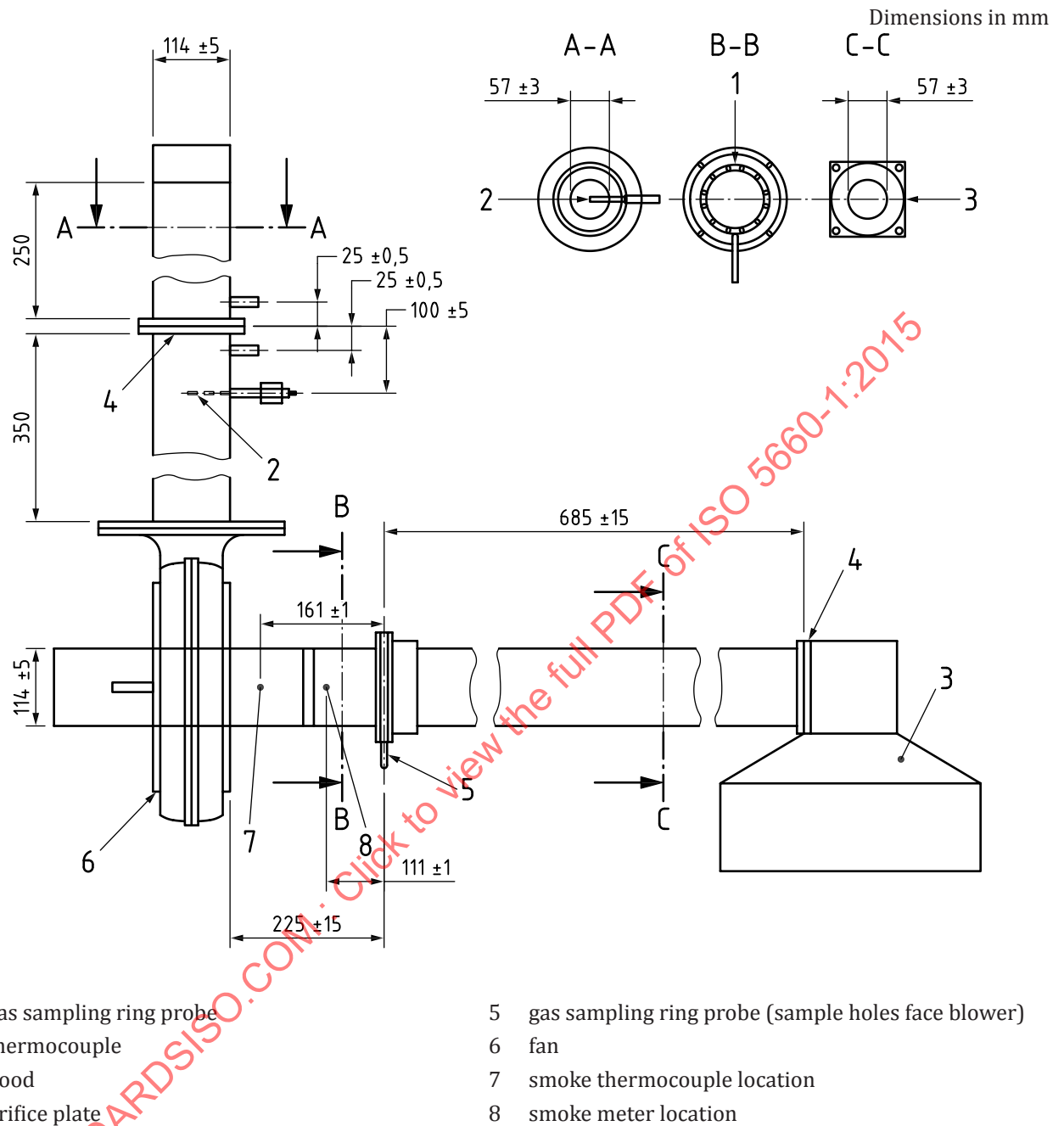
Figure 5 — Exhaust system
