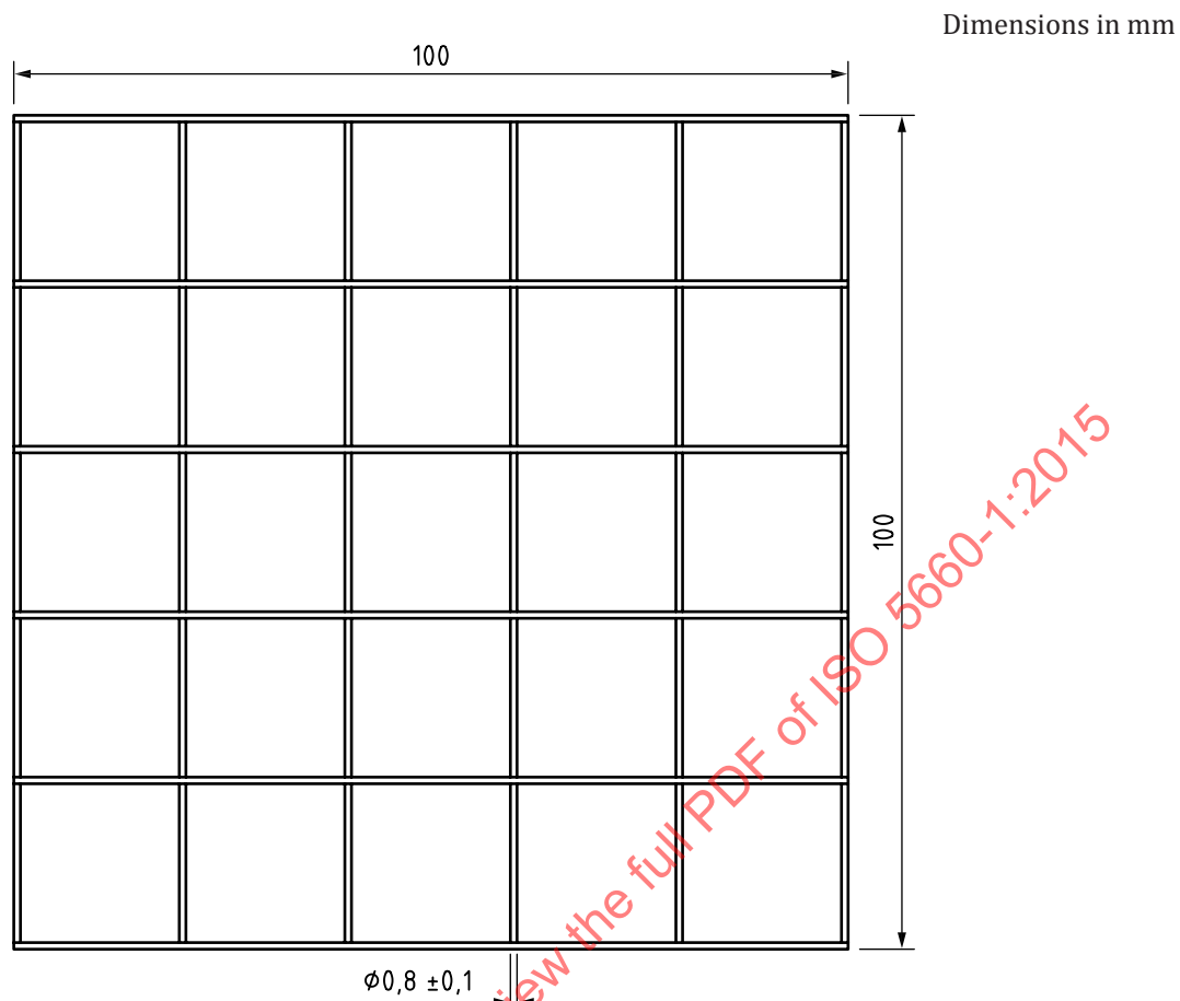
Figure 8 — Fine wire grid
