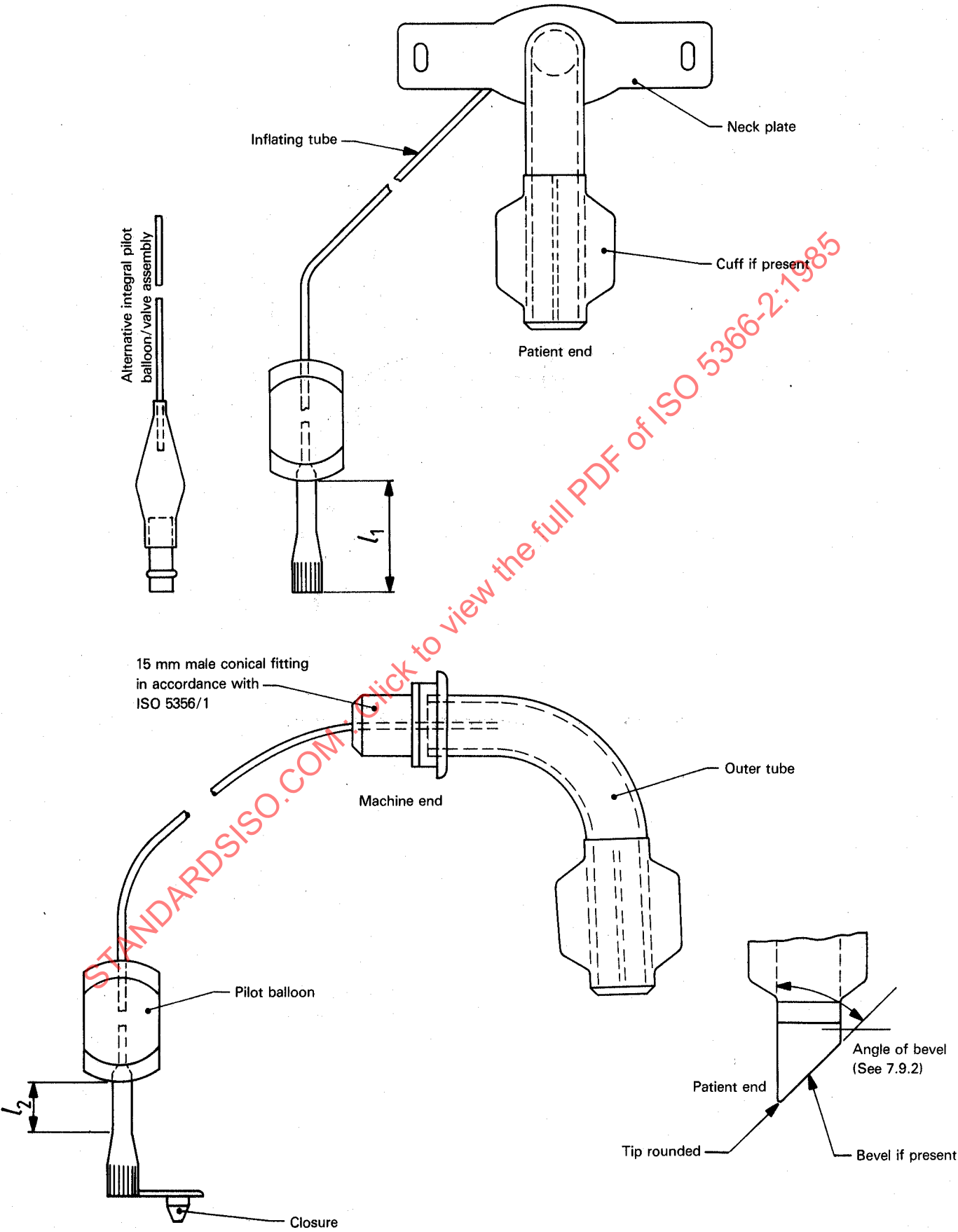
Figure 1 – Typical tracheostomy tube
