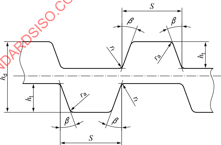
Figure 3 — Tooth profile, double-sided — Type B
