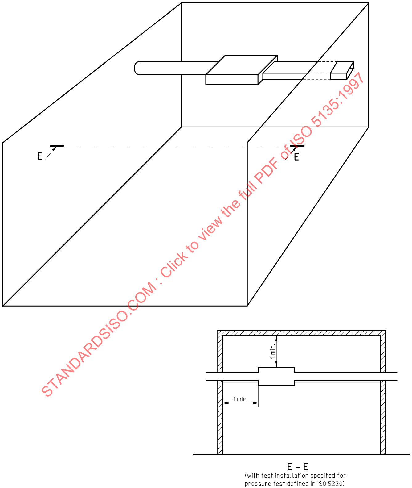
Figure 6 — Mounting detail for air-terminal unit to determine casing radiated sound
