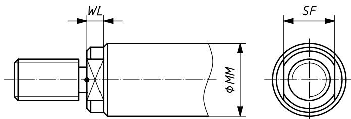
Figure 4 — Wrench flats for a hydraulic cylinder piston rod end (male thread)
