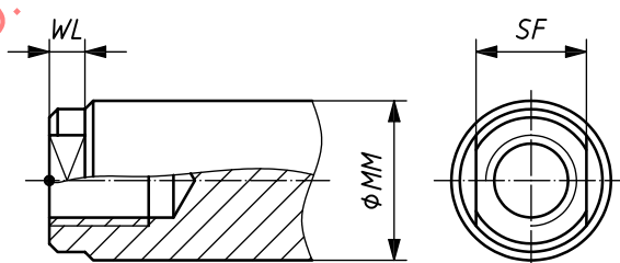
Figure 6 — Wrench flats for a hydraulic cylinder piston rod end (female thread)
