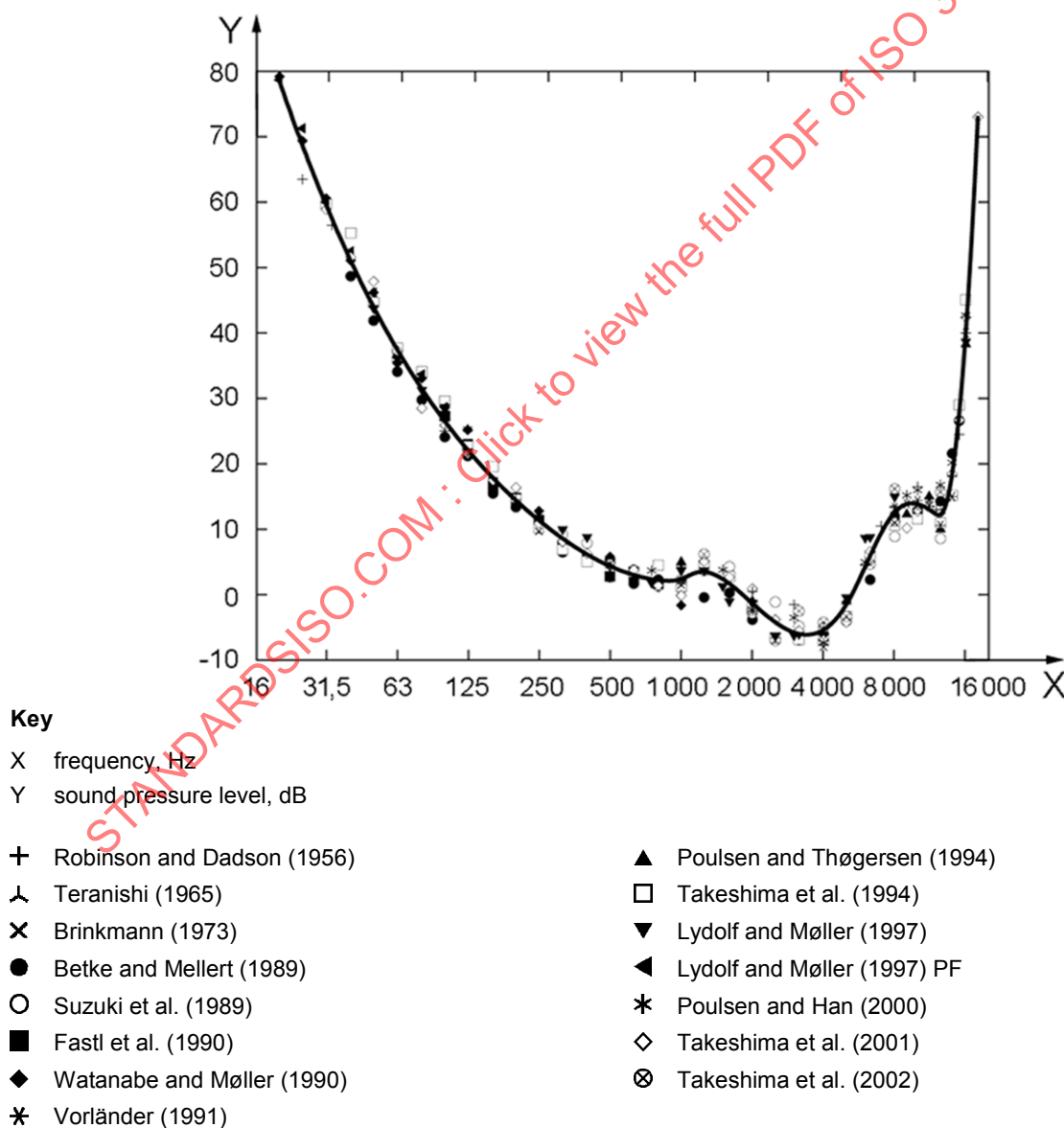
Figure A.1 — Experimental data used for the derivation of the reference thresholds of hearing under free-field listening conditions and the calculated curve giving best fit to these data
