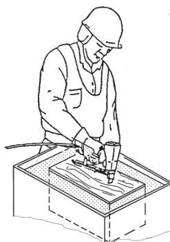
Figure 11 — Fastener driving tool — Working position of operator
