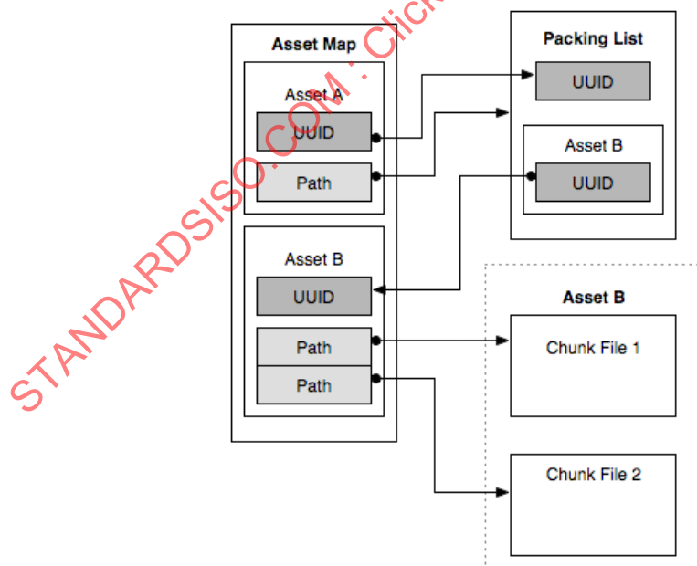
Figure 1 – Relationship between the Packing List and Asset Map structures
