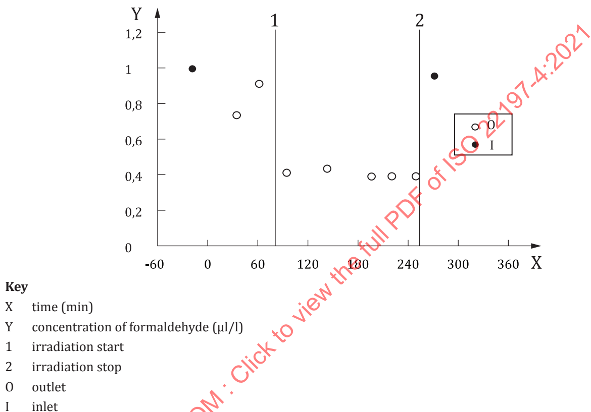
Figure 3 — Typical trace of formaldehyde concentration during the test operation
