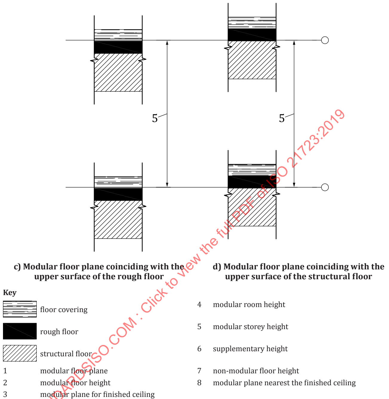
Figure 1 — Different positions of the modular floor plane
