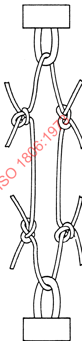
FIGURE 2 — Mounting of a mesh by loops
