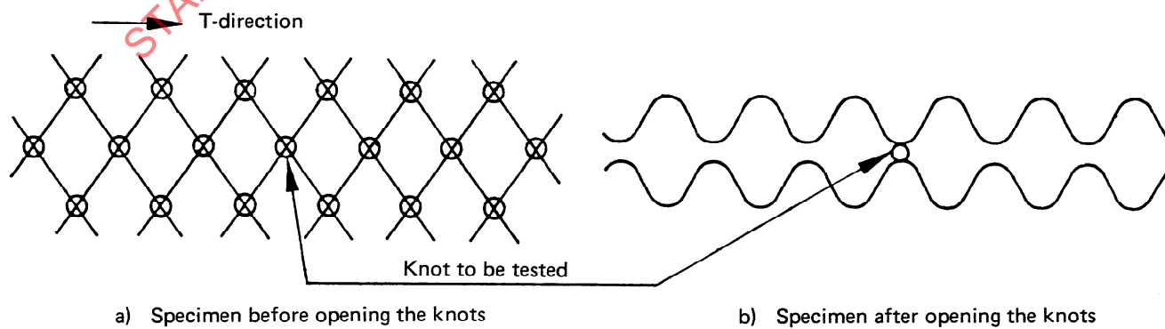
FIGURE 3 — Preparation of specimen for determination of knot breaking load
