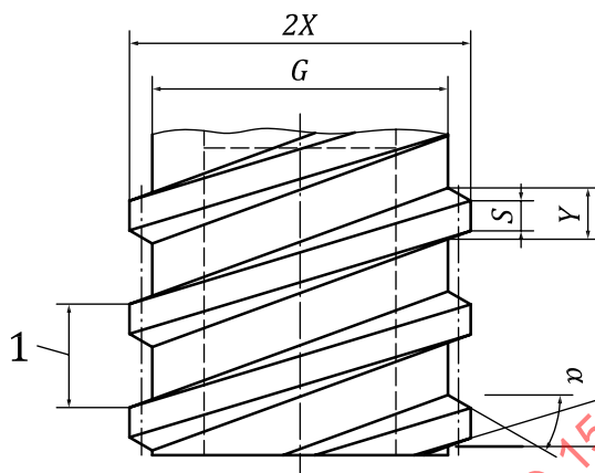
Figure B.8 — Female 6 % (Luer) conical lock fittings with lugs in a plane at right angles to axis of fitting
