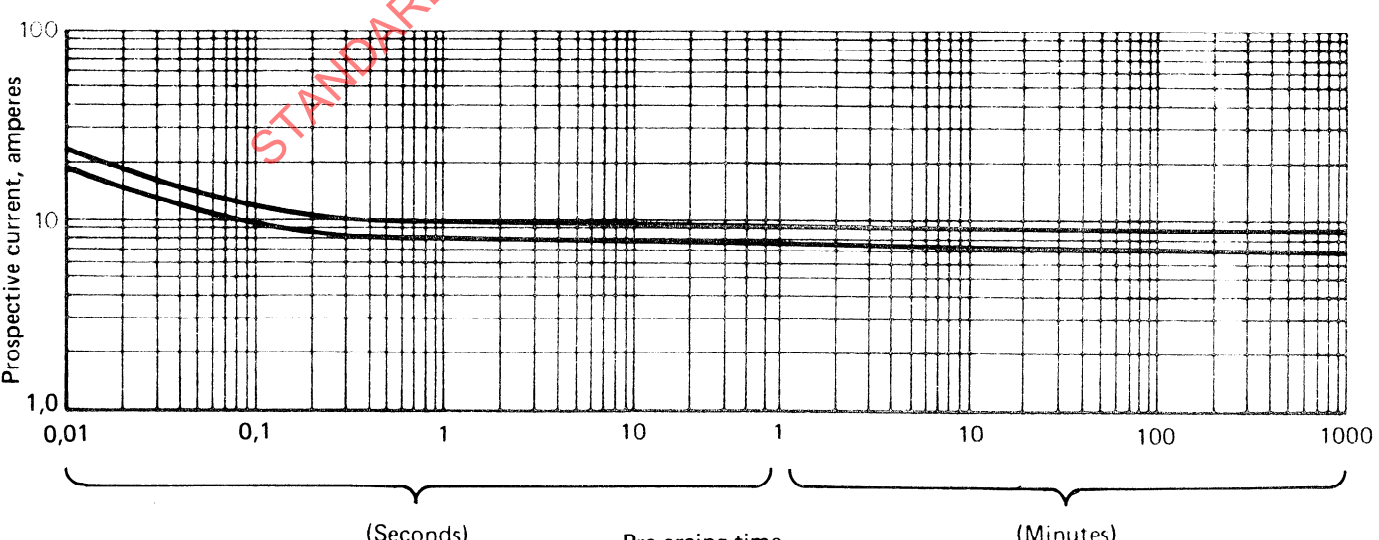
FIGURE 5 – Type B.1; 5 A
