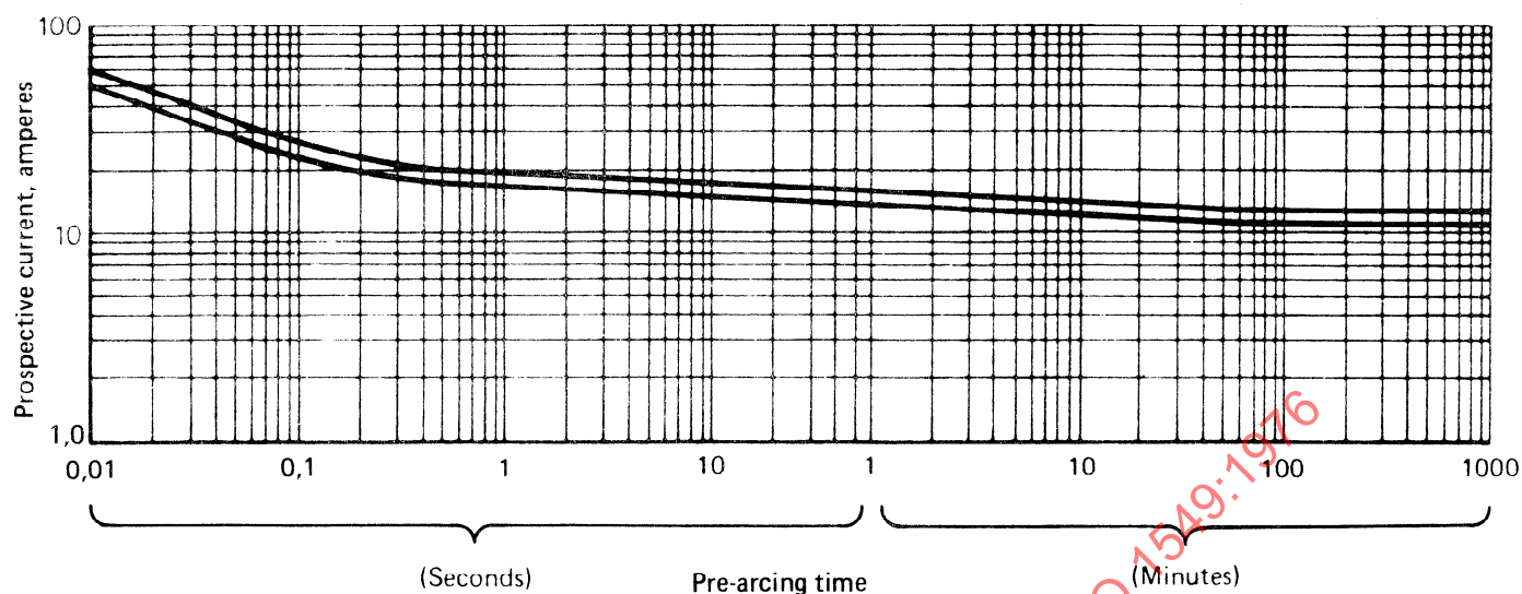
FIGURE 6 – Type B.1; 7,5 A
