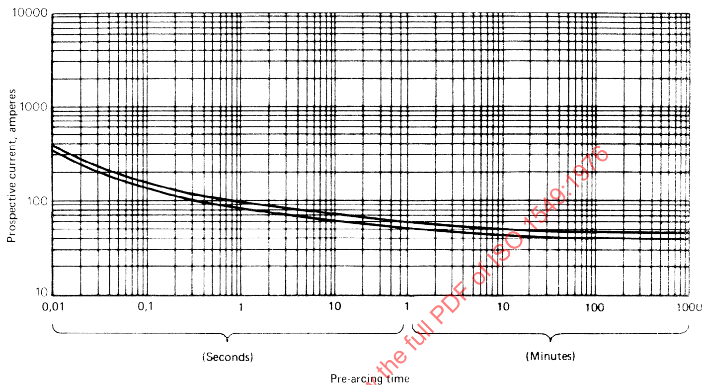
FIGURE 11 Type B.6; 30 A
