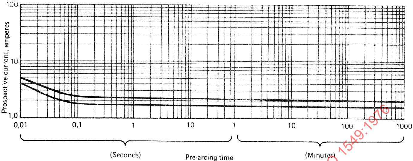
FIGURE 3 – Type B.1; 1 A
