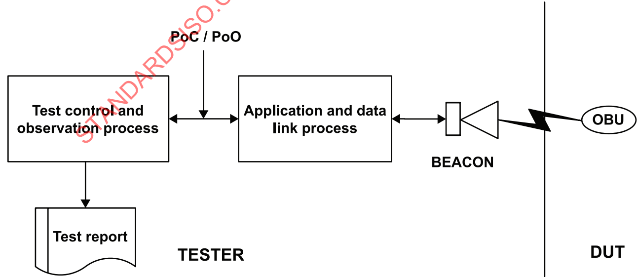
Figure 5 — Test facilities
