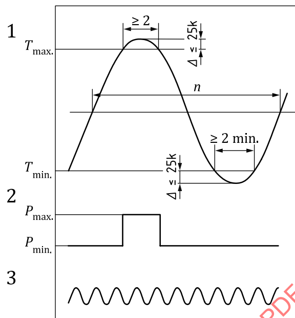
Principle PTV test method 1
