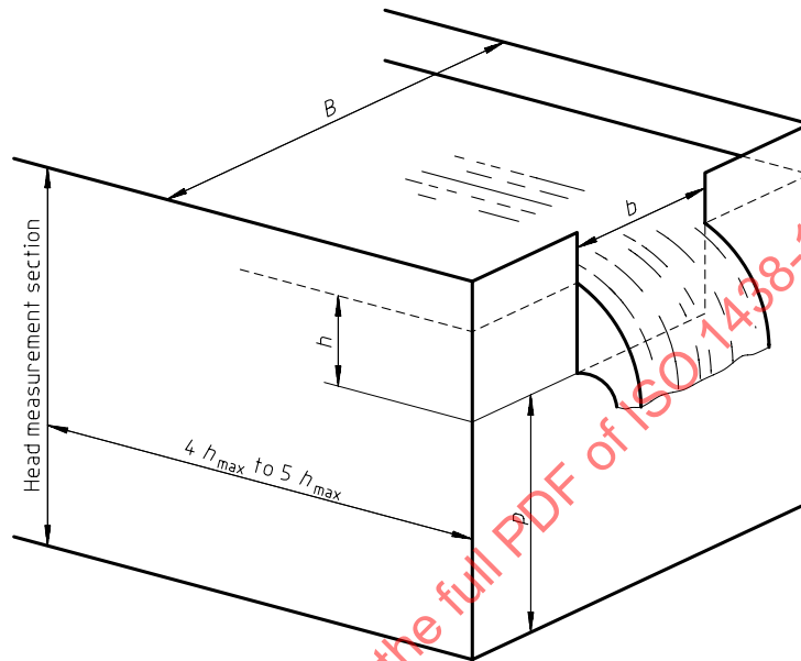
Figure 2 — Rectangular-notch thin-plate weir
