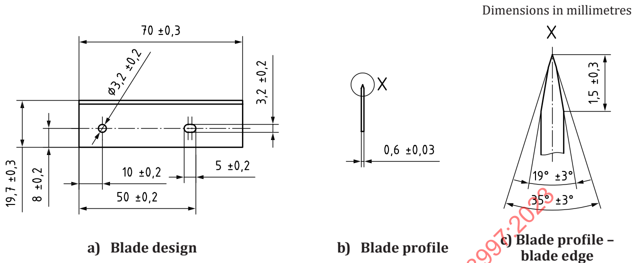
Figure 7 — Examples of blade design
