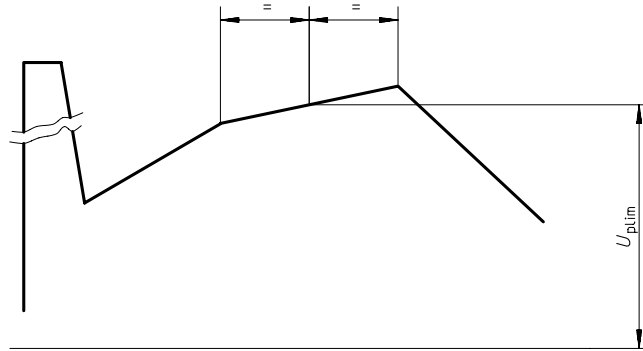
Figure 4 — Primary clamp voltage ( U_{plim} )
