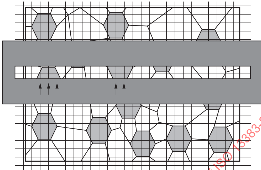
Figure 1 — Schematic diagram of microstructure overlaid with square grid and with optional screen applied. Intersections of the grid with the dark phase are arrowed
