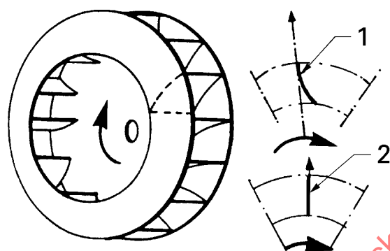
Radial-tipped
