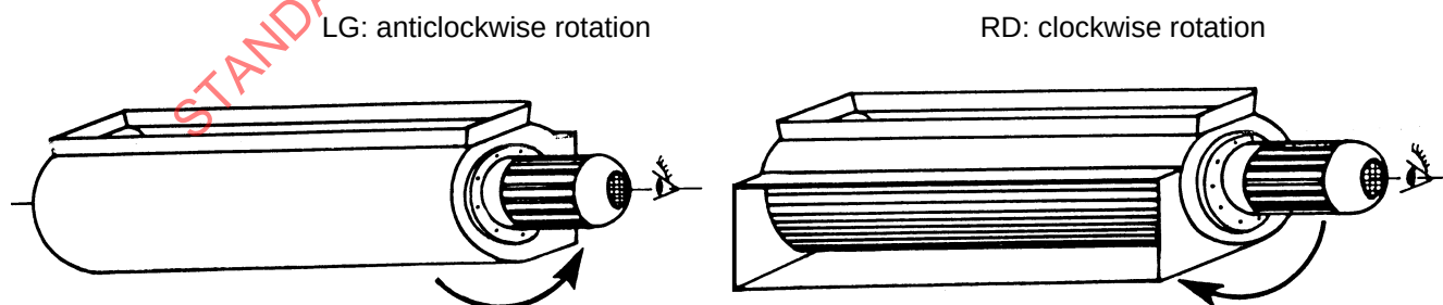
Figure 17 — Direction of rotation of cross-flow fans
