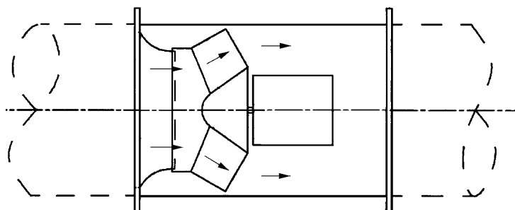
Figure 5 — Mixed-flow fan
