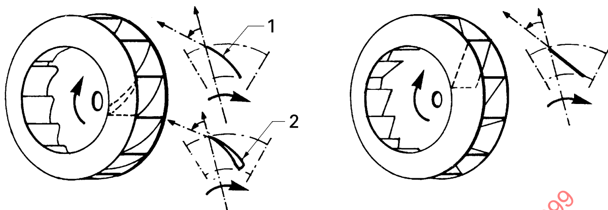
Backward-curved
