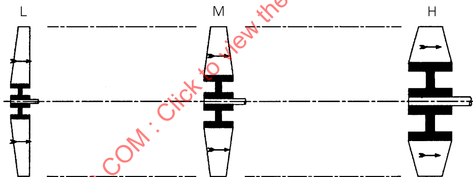
Figure 10 — Impellers of an axial-flow fan
