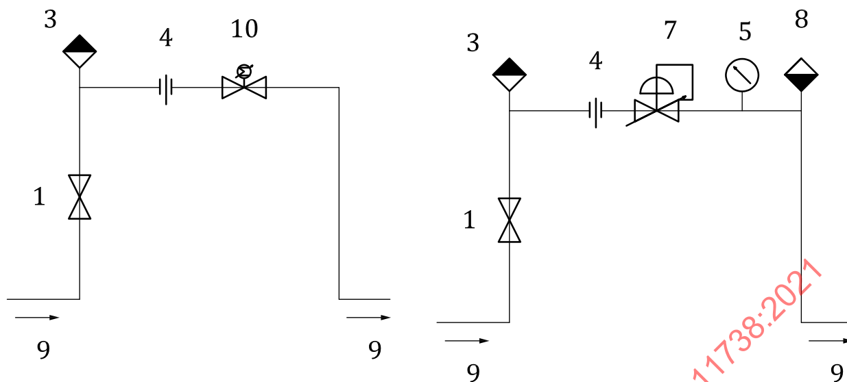
a) Irrigation control head for automation with volumetric valve or metering
