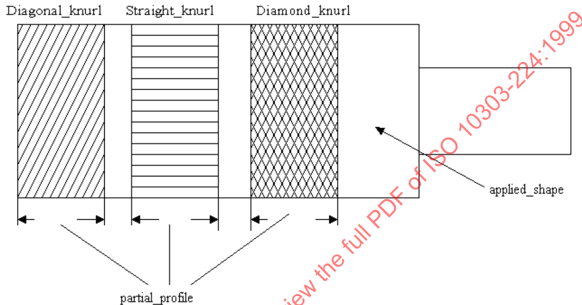
Figure 57 - Knurl
