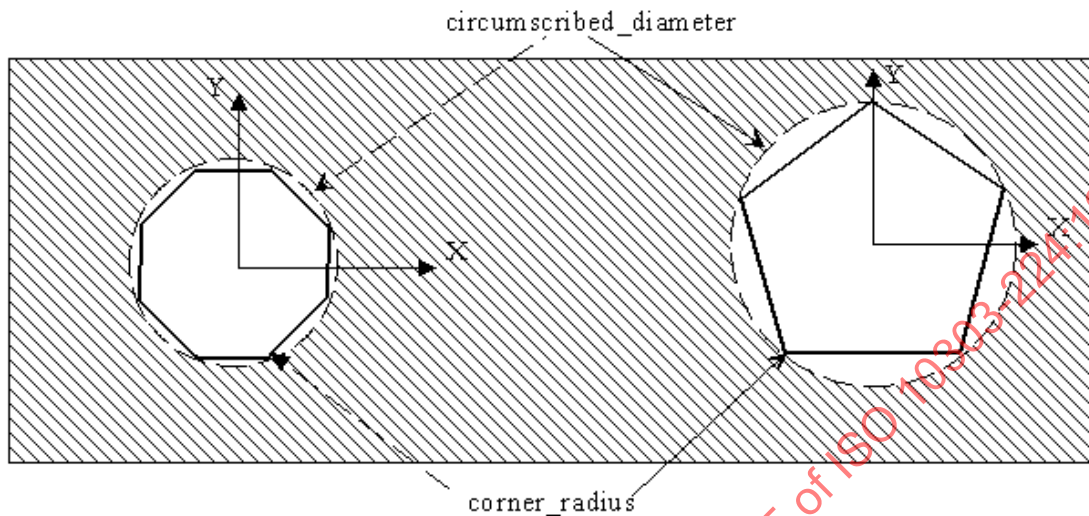
Figure 63 - Ngon_profile
