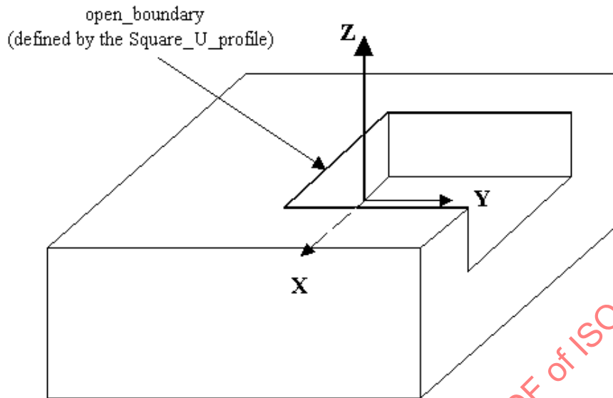
Figure 81 - Rectangular_open_pocket
