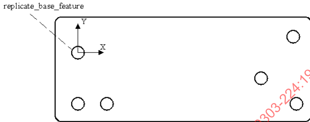
Figure 50 - General_pattern
