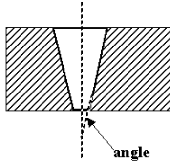
Figure 2 - Angle_taper
