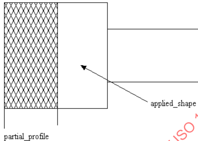
Figure 38 - Diamond knurl
