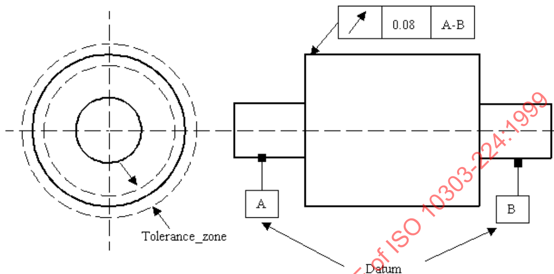
Figure 20 - Circular_runout_tolerance
