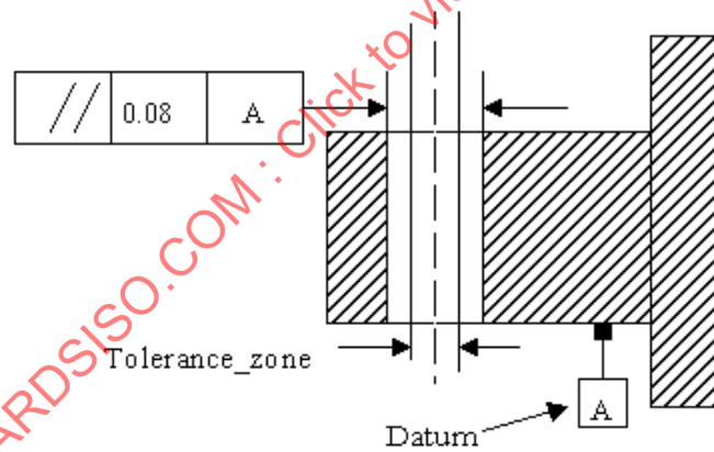
Figure 68 - Parallelism_tolerance for an axis
