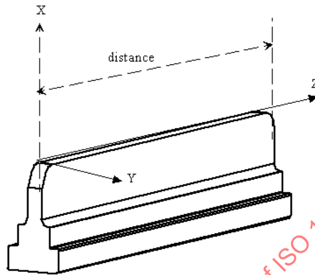
Figure 58 - Linear_path
