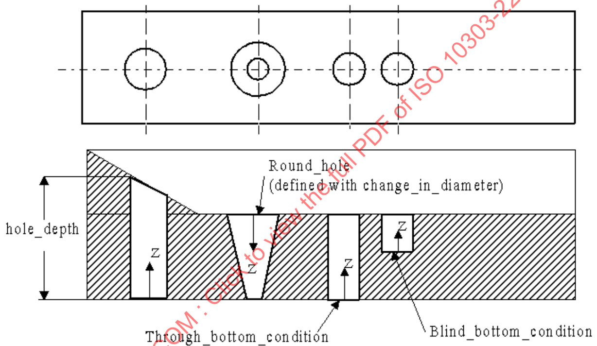
Figure 85 - Round_hole
