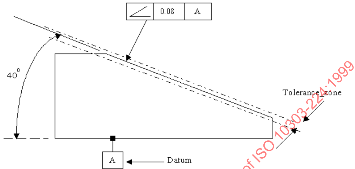
Figure 6 - Angularity_tolerance for a plane surface
