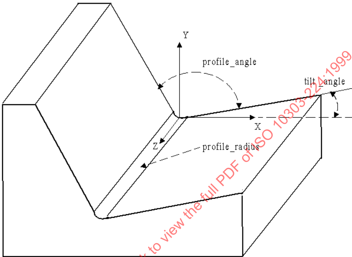
Figure 102 - Vee_profile
