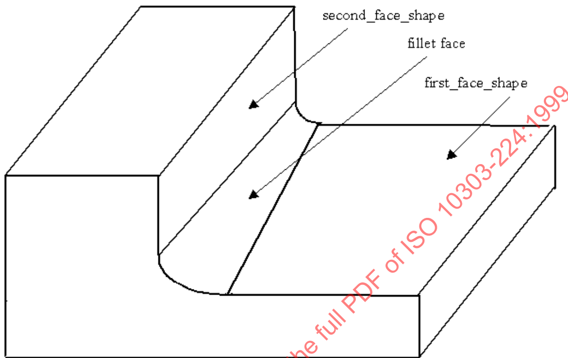
Figure 41 - Fillet
