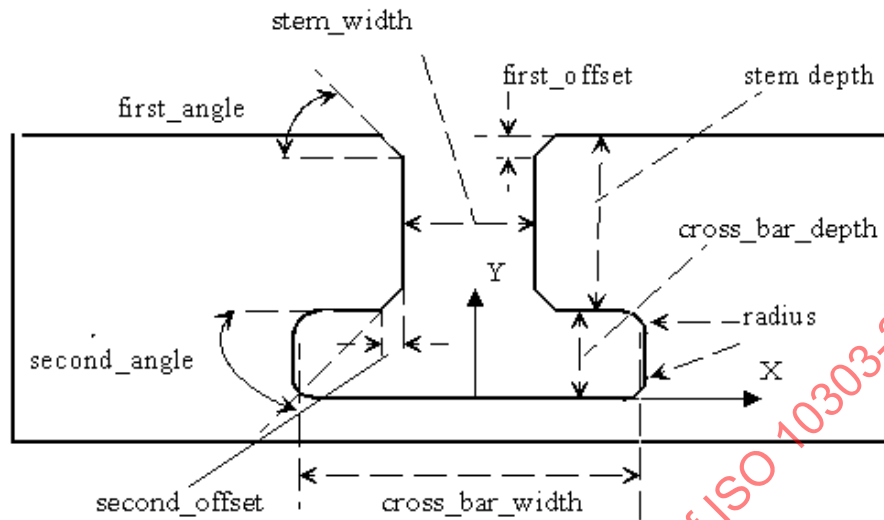
Figure 97 - Tee_profile
