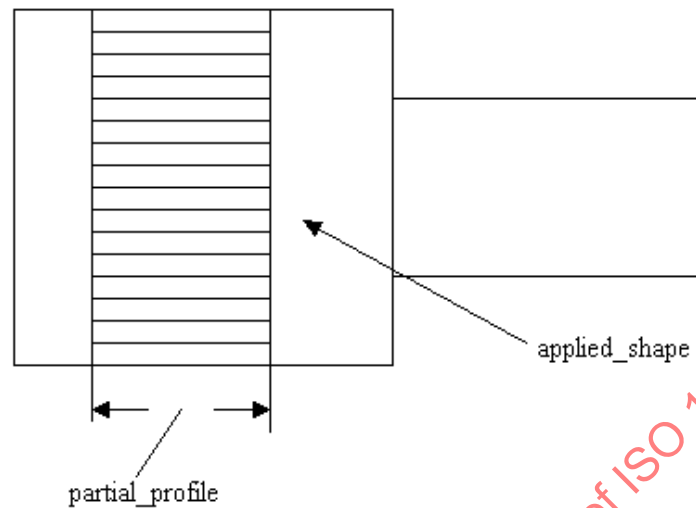
Figure 93 - Straight_knurl
