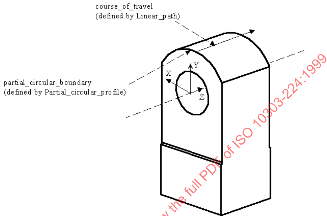
Figure 86 - Rounded_end
