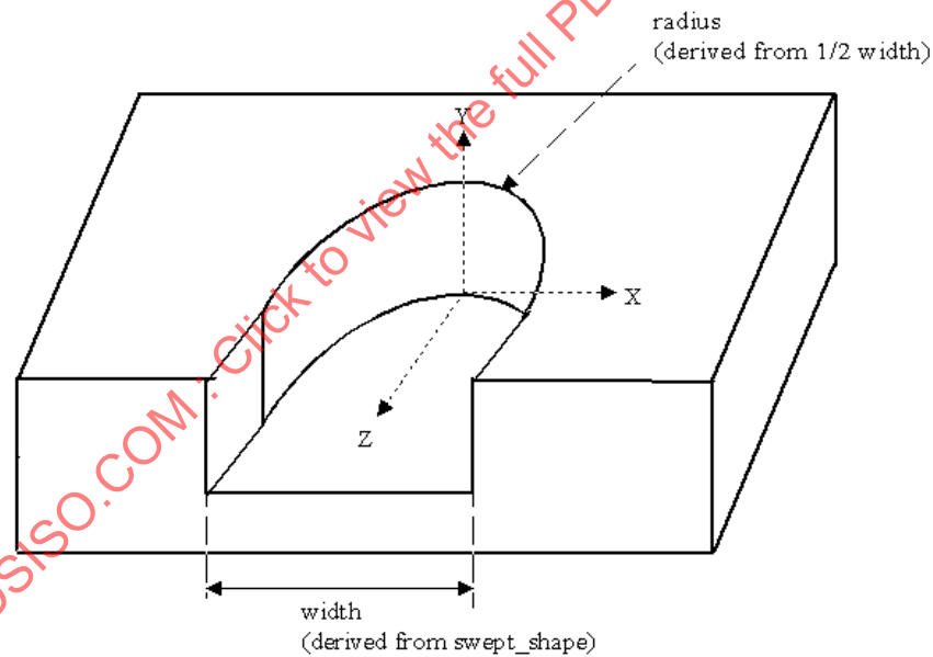
Figure 76 - Radiused_slot_end_type
