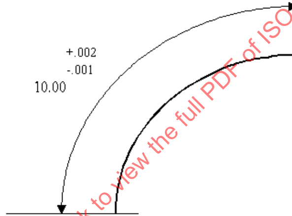
Figure 30 - Curved_dimension_tolerance
