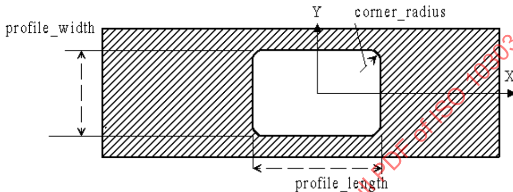
Figure 78 - Rectangular_closed_profile
