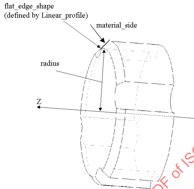
Figure 83 - Revolved_flat
