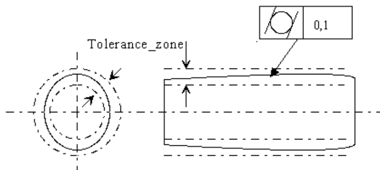
Figure 32 - Cylindricity_tolerance
