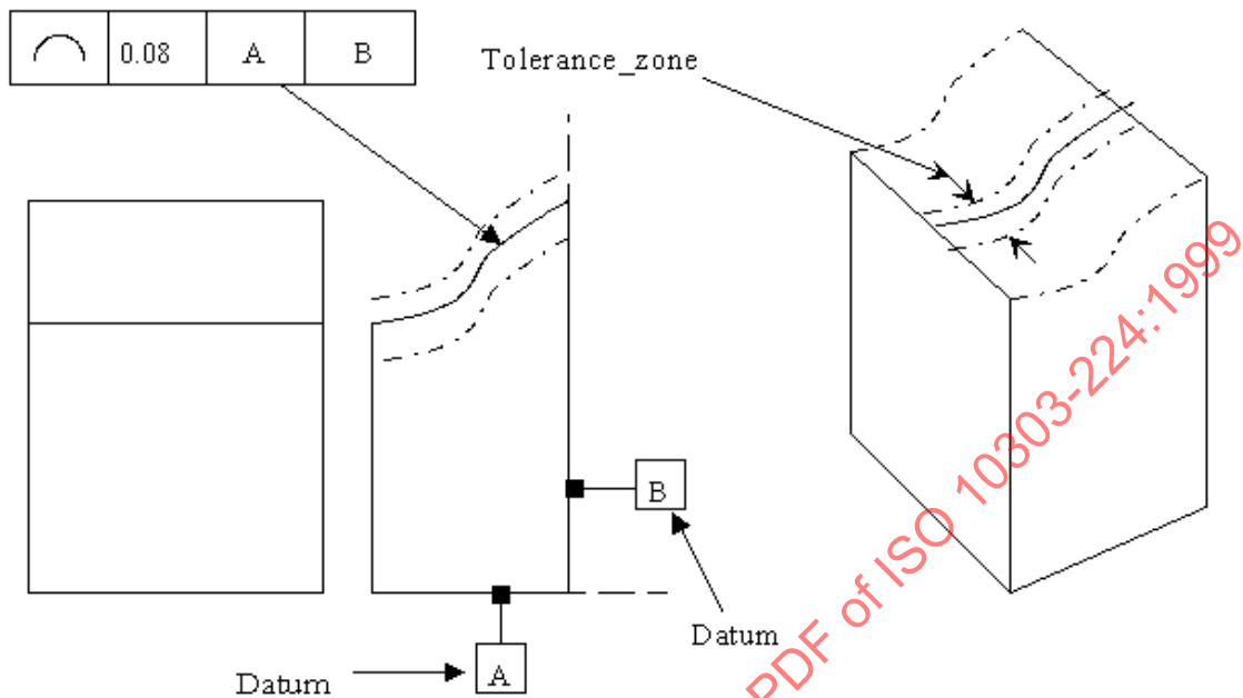
Figure 60 - Linear_profile_tolerance
