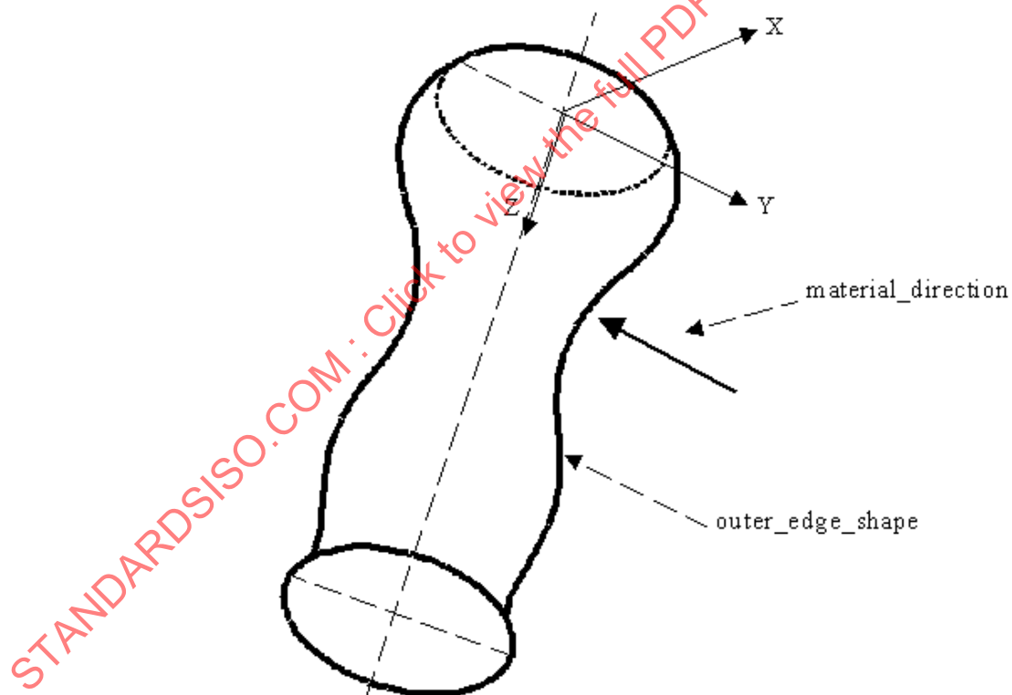
Figure 53 - General_revolution for outer shape
