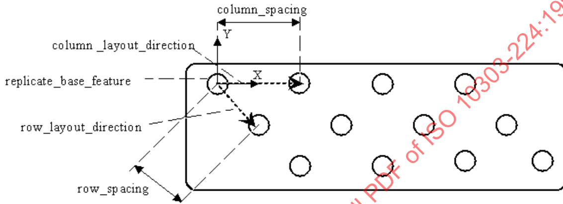
Figure 82 - Rectangular_pattern
