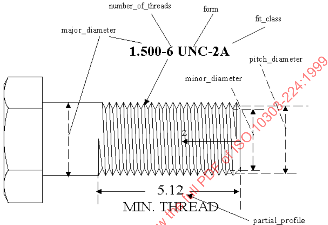
Figure 34 - Thread and Defined_thread attributes
