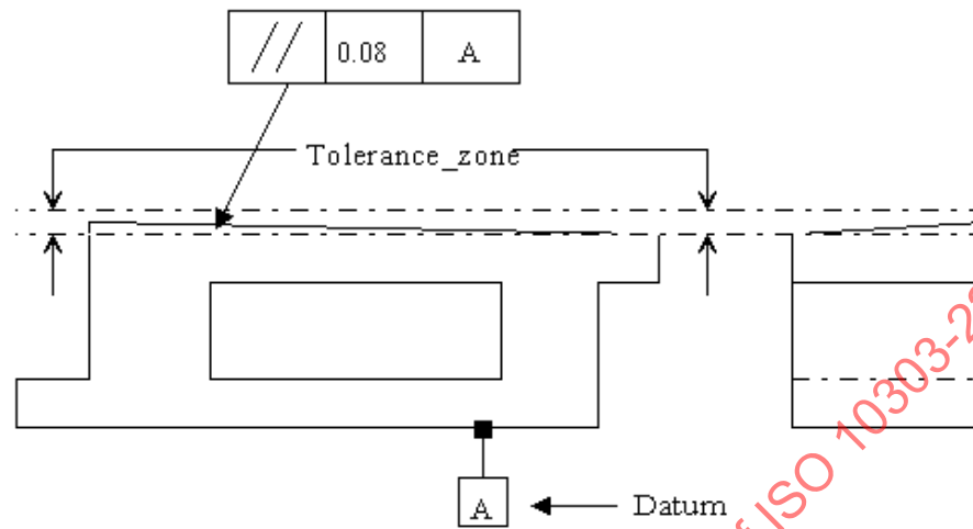
Figure 67 - Parallelism_tolerance for a plane
