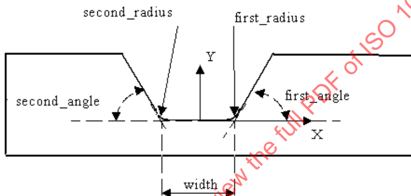
Figure 91 - Square_U_profile
