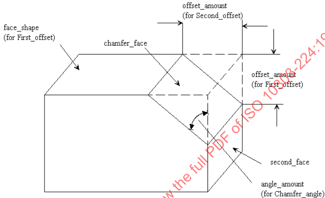
Figure 12 - Chamfer
