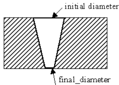
Figure 37 - Diameter_taper
