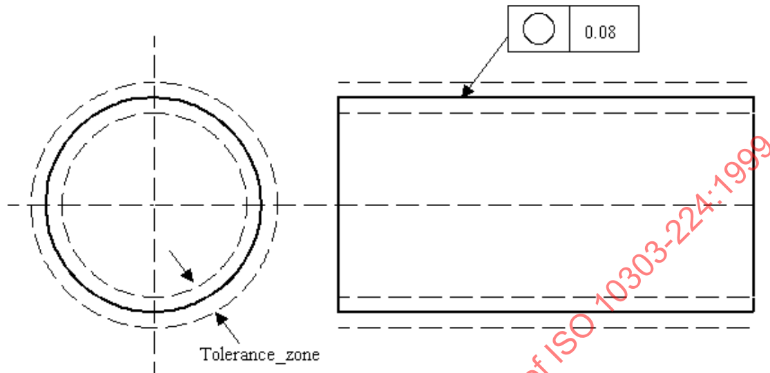
Figure 21 - Circularity tolerance
