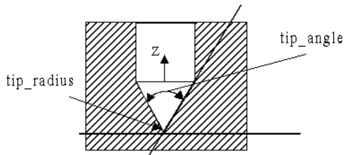
Figure 25 - Conical_hole_bottom
