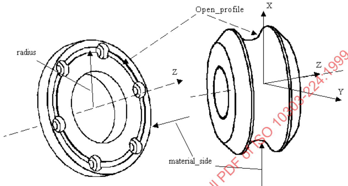
Figure 55 - Groove
