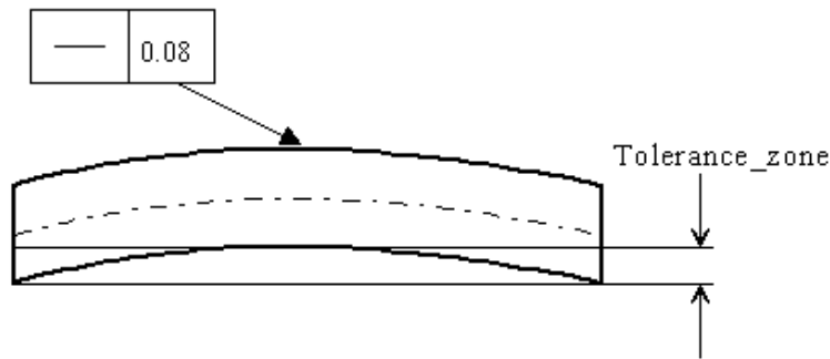
Figure 94 - Straightness_tolerance
