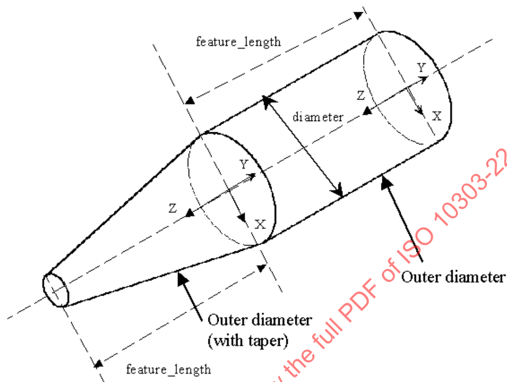
Figure 65. Outer_diameter
