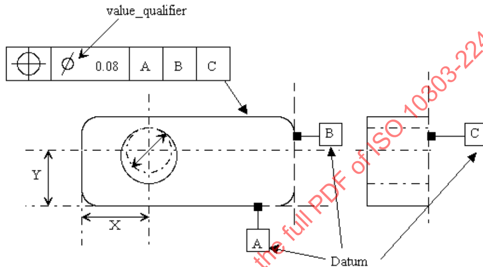
Figure 73 - Position_tolerance
