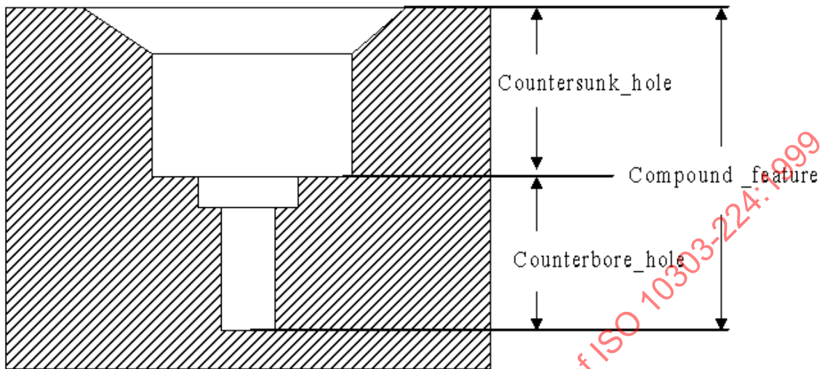
Figure 23 - Compound_feature
