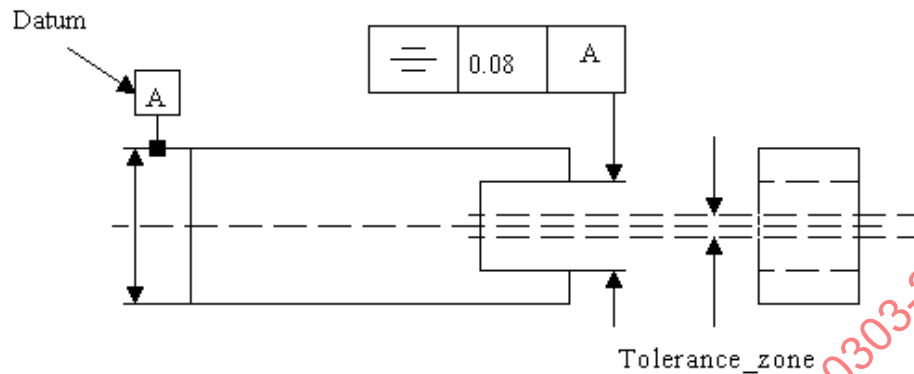
Figure 96 - Symmetry_tolerance
