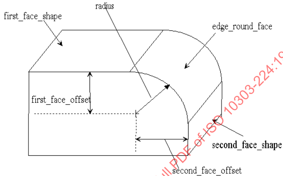
Figure 26 - Constant_radius_edge_round
