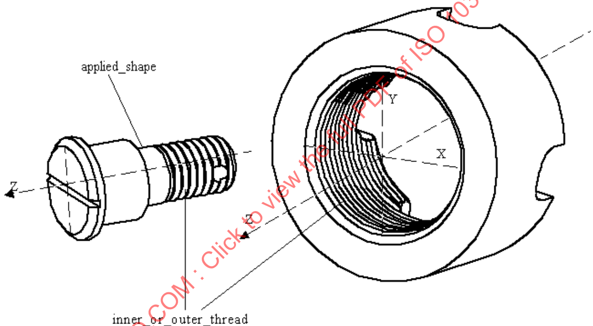
Figure 98 - Thread
