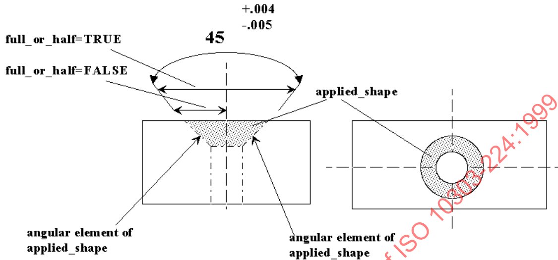
Figure 5 - Angular_size_dimension_tolerance
