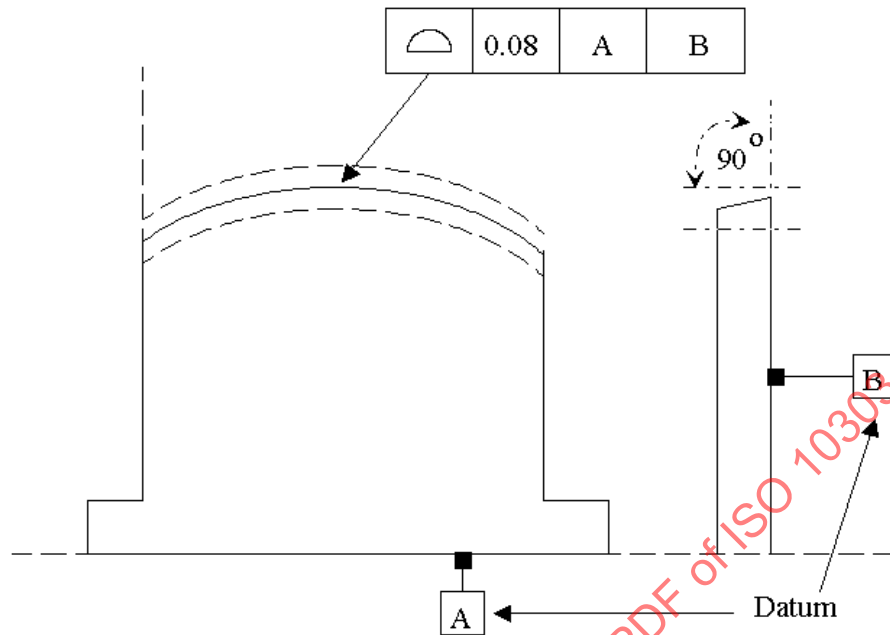
Figure 95 - Surface_profile_tolerance
