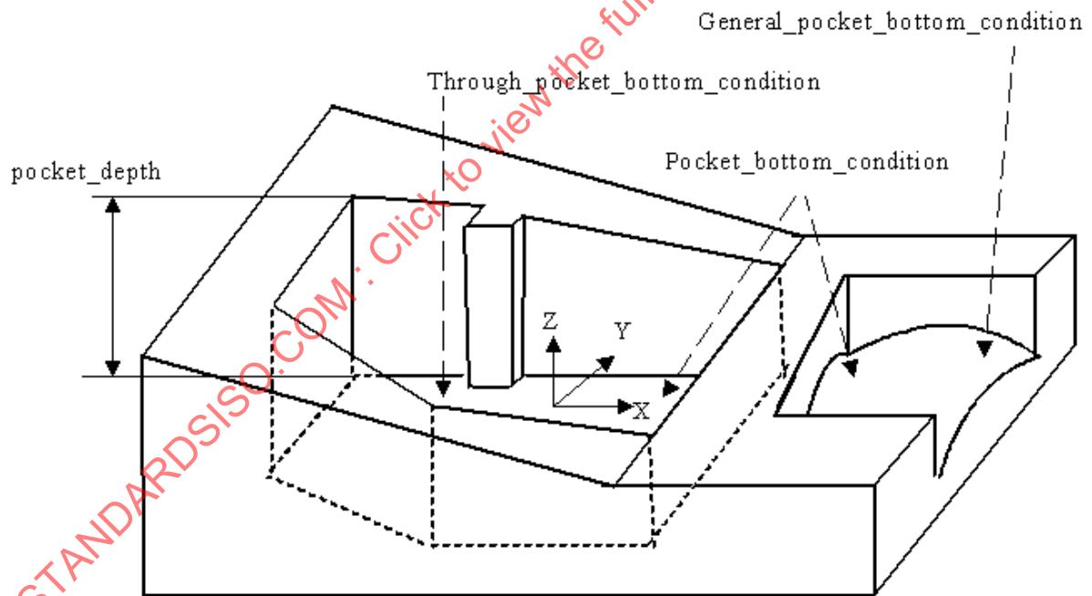
Figure 51 - General_pocket
